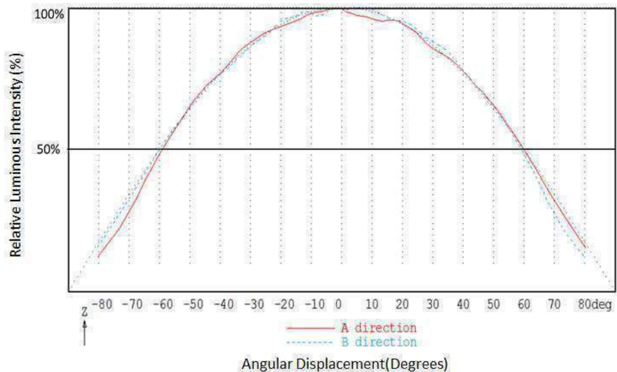
Figure 4 Radiation Diagram
