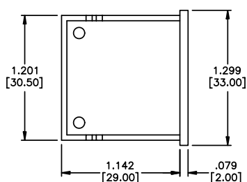
DPS10L2 Dummy housing
