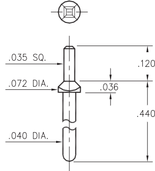
8953-0-05-XX-00-00-03-0 Square press-fit in .047 plated thru hole
