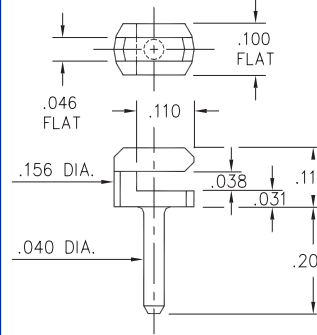
7310-0-01-XX-00-00-08-0 Board edge press-fit
