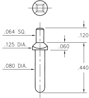
8952-0-05-XX-00-00-03-0 Square press-fit in .087 plated thru hole
