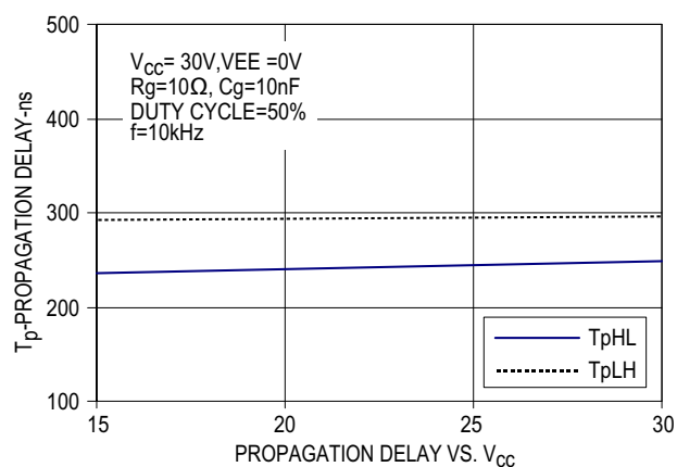
Figure 10 Propagation Delay vs. V_{CC}
