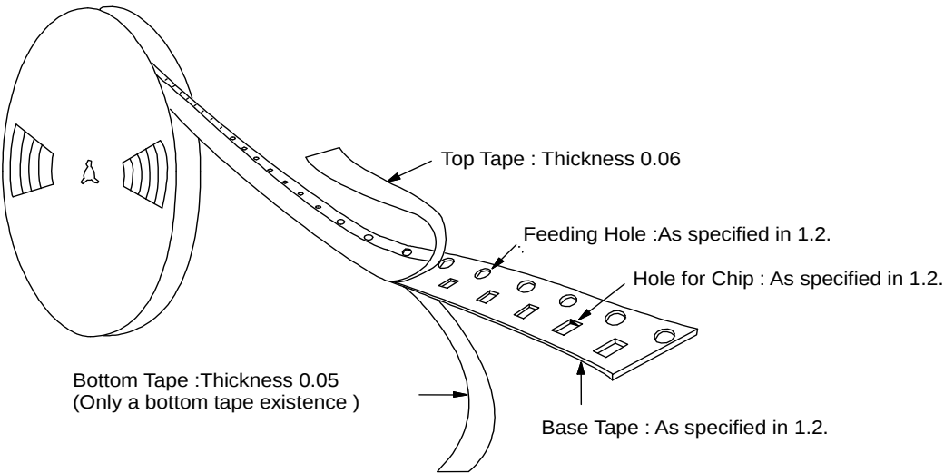
Fig.3 Taping Diagram
