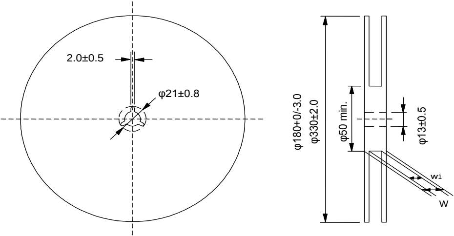
Fig.3 Taping Diagram
