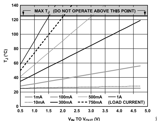
Figure 41. 0 mm 2 of PCB Copper, T_A = 25^\circ\text{C} , LFCSP
