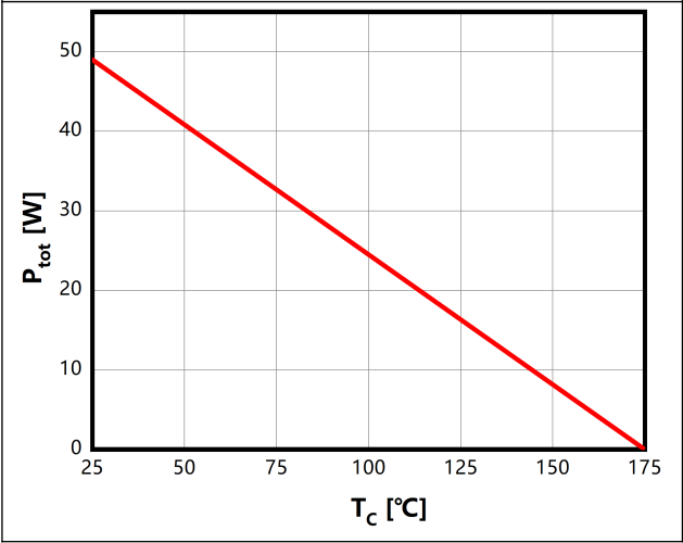
Figure 6. Power Derating
