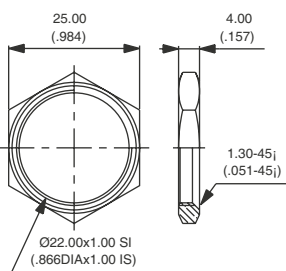
HEX NUT FOR MODELS Ø 22 (.866)
