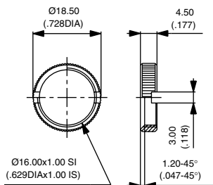
KNURLED NUT FOR MODELS Ø 16 (.629)
