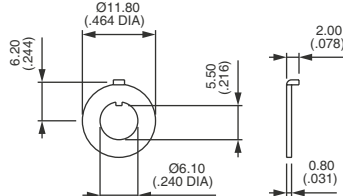
Nickel plated U198 Black U728
