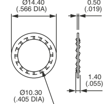
Zinc plated steel U843
