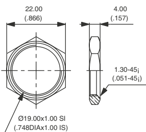
HEX NUT FOR MODELS Ø 19 (.748)
