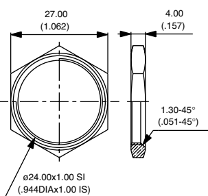
HEX NUT FOR MODELS Ø 24 (.944)
