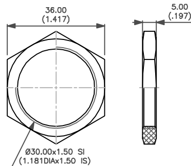
HEX NUT FOR MODELS Ø 30 (1.181)
