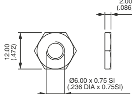
Chrome plated U1916
