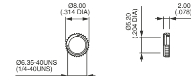
Chrome plated U501
