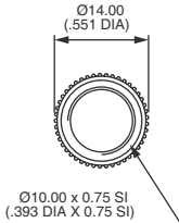
Nickel plated U2311
