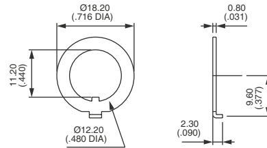
Nickel plated U121 Black U12
