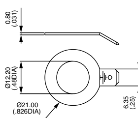
Nickel plated U187
