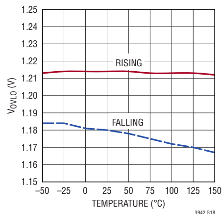
OVLO Threshold
