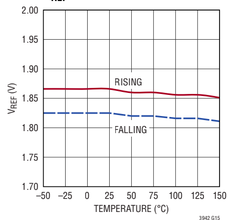
V REF UVLO Threshold
