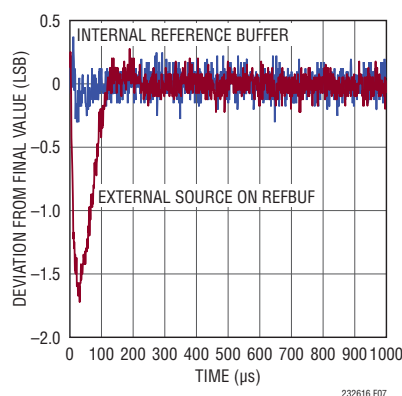
Figure 7. Transient Response of the LTC2326-16
