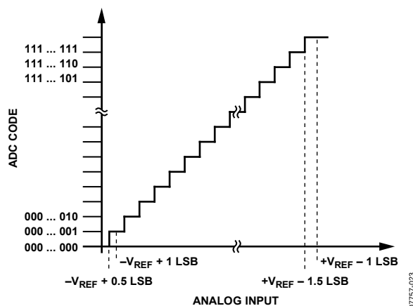
Figure 24. Ideal Transfer Characteristic
