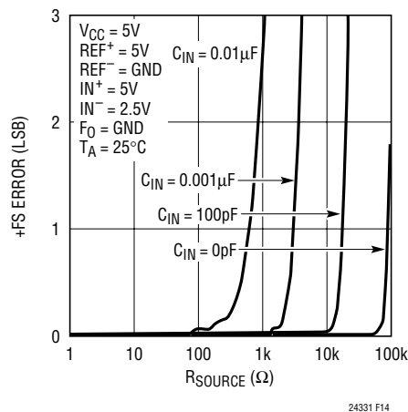
Figure 14. +FS Error vs R_{SOURCE} at \text{IN}^+ or \text{IN}^- (Small C_{IN} )
