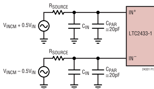
Figure 13. An RC Network at \text{IN}^+ and \text{IN}^-
