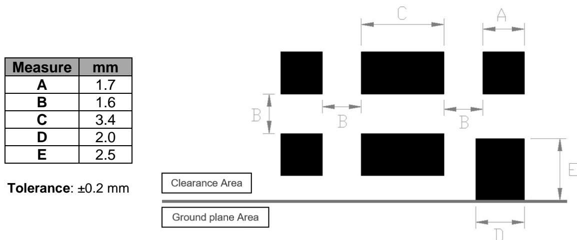
Figure 9 – Footprint dimensions for the double booster.
