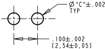
RECOMMENDED HOLE PATTERN GAUGE
