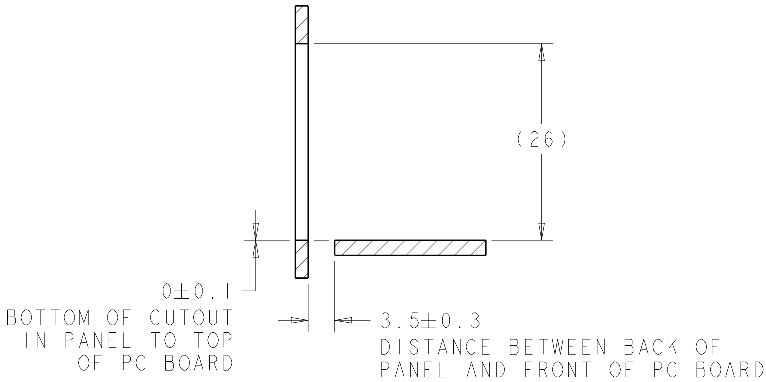
SECTION U-U
