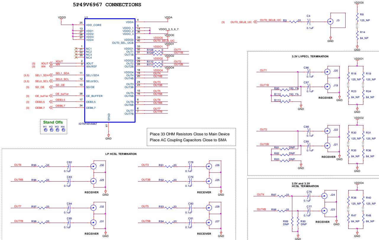
Figure 11. 5P49V6967 Evaluation Board Schematics – Page 2
