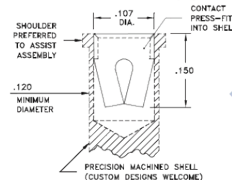
#07 CONTACT FOR .065"-.082" DIAMETER PINS ( \delta = .013 ) 4-FINGER, GROUP H (See page 248)
