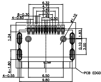
PCB LAYOUT TOLERANCESIZE:±0.05
