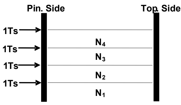
Figure 4—Winding Diagram
