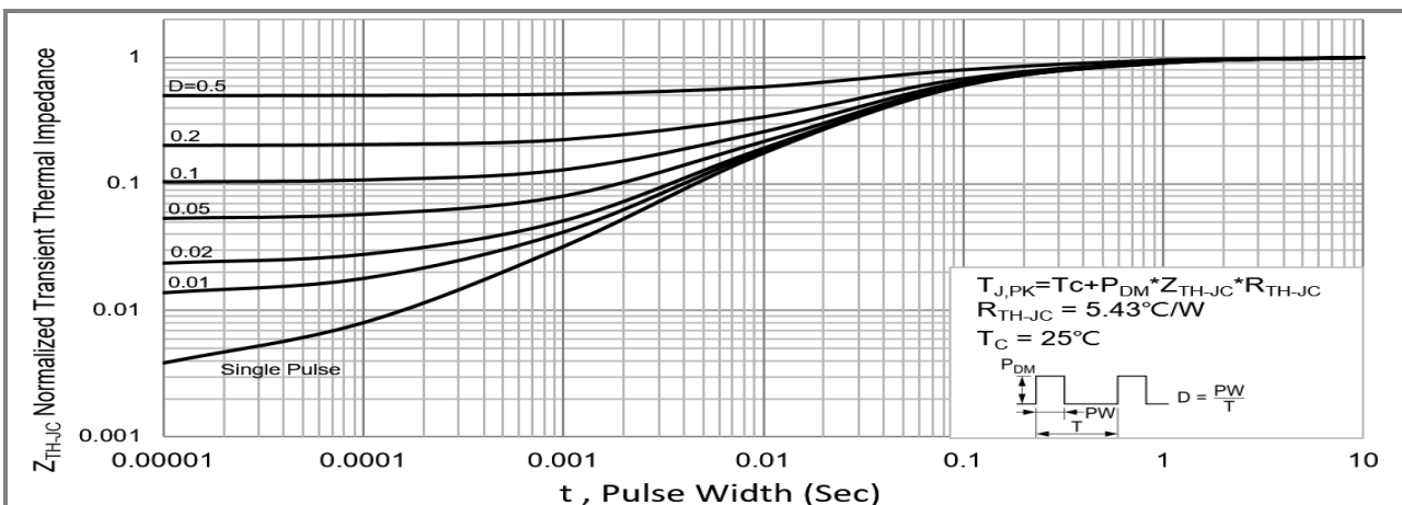
Fig.15 PJF3NA50 Normalized Transient Thermal Impedance vs. Pulse Width
