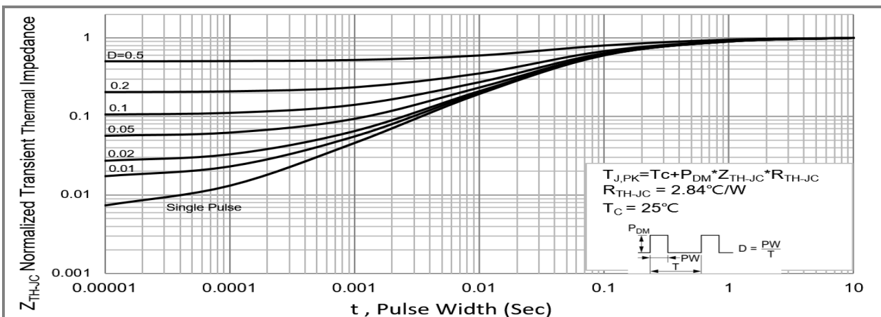
Fig.14 PJP3NA50 Normalized Transient Thermal Impedance vs. Pulse Width
