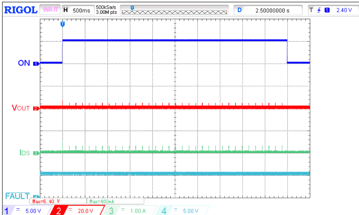
Figure 23. Typical SOA waveform during power up under heavy load for V IN = 24 V, C LOAD = 10 μF, R SET = 30.1 kΩ, R LOAD = 12 Ω
