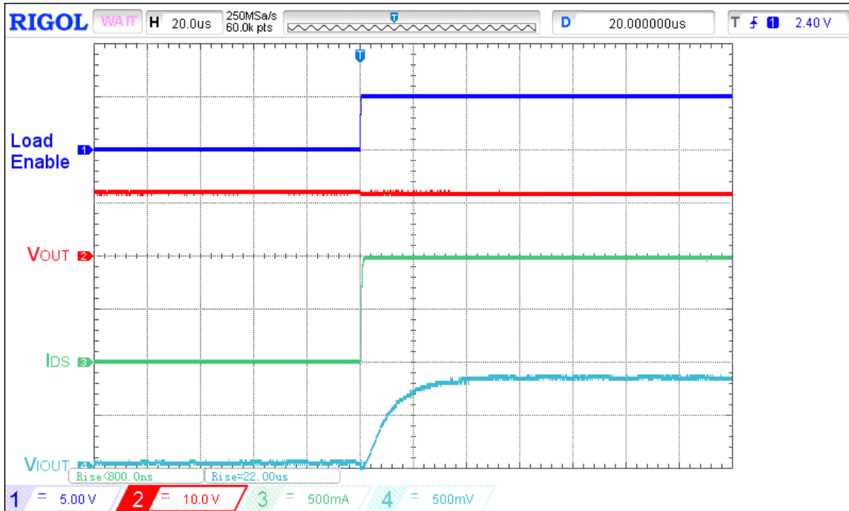
Figure 17. Typical I OUT response time waveform for V IN = 12 V, C LOAD = 10 μF, R LOAD = 12 Ω C IOUT = 0.18 nF, R IOUT = 84.5 kΩ, Load step 0 A to 1 A
