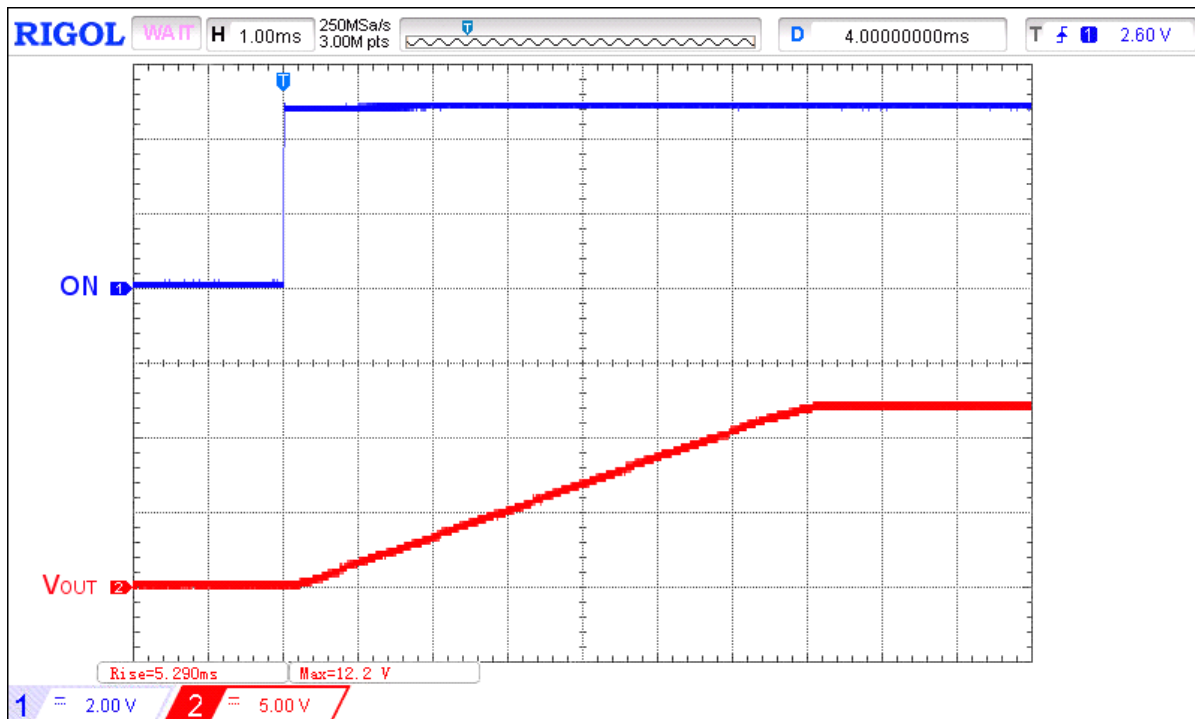
Figure 3. Typical Turn ON operation waveform for V_{IN} = 12 V, C_{SLEW} = 18 nF, C_{LOAD} = 10 μF, R_{LOAD} = 100 Ω
