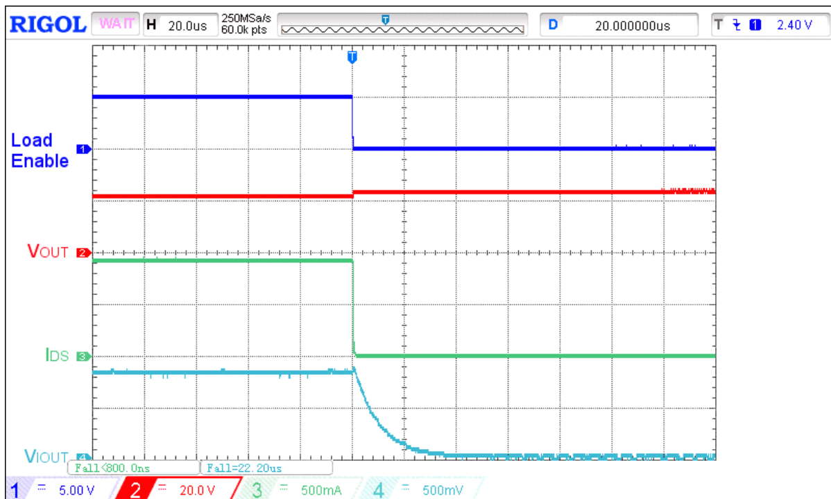
Figure 20. Typical I_{OUT} response time waveform for V_{IN} = 24 V, C_{LOAD} = 10 \mu F, R_{LOAD} = 24 \Omega C_{IOUT} = 0.18 nF, R_{IOUT} = 84.5 k \Omega , Load step 1 A to 0 A
