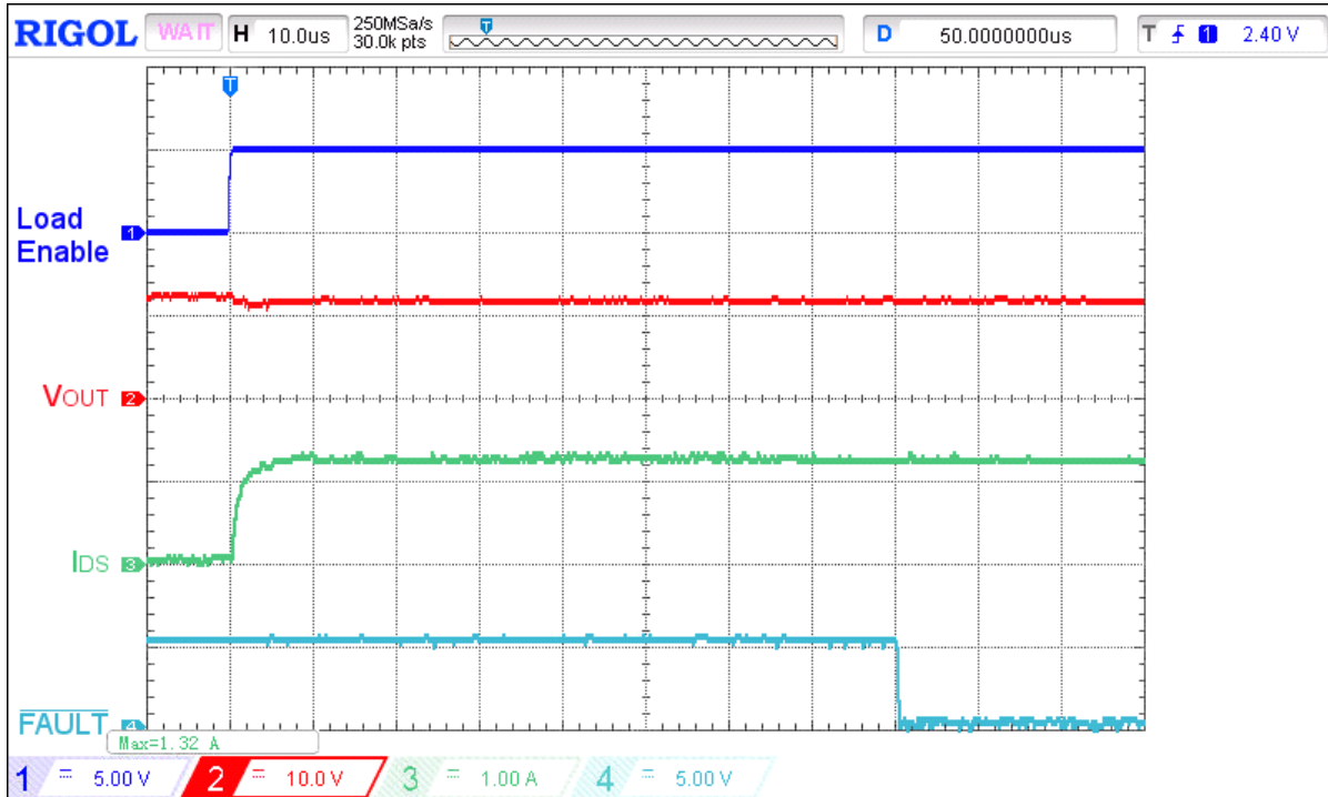
Figure 13. Typical FAULT assertion waveform for V IN = 12 V, C LOAD = 10 μF, I ACL = 1 A, R SET = 91 kΩ, switch on 9 Ω load
