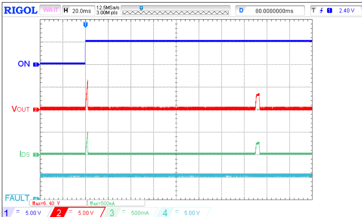
Figure 24. Extended typical SOA waveform during power up under heavy load for V IN = 24 V, C LOAD = 10 μF, R SET = 30.1 kΩ, R LOAD = 12 Ω
