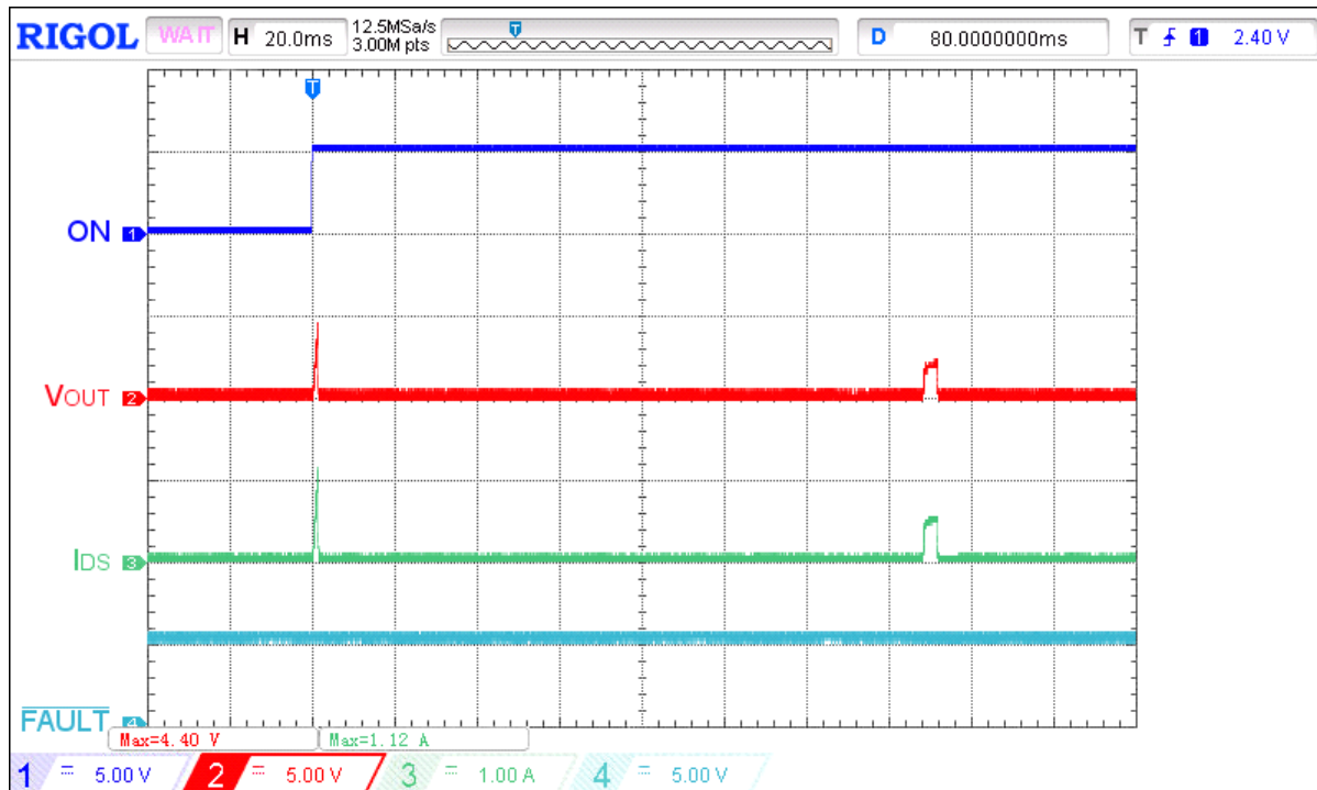
Figure 22. Extended typical SOA waveform during power up under heavy load for V IN = 12 V, C LOAD = 10 μF, R SET = 30.1 kΩ, R LOAD = 3.5 Ω
