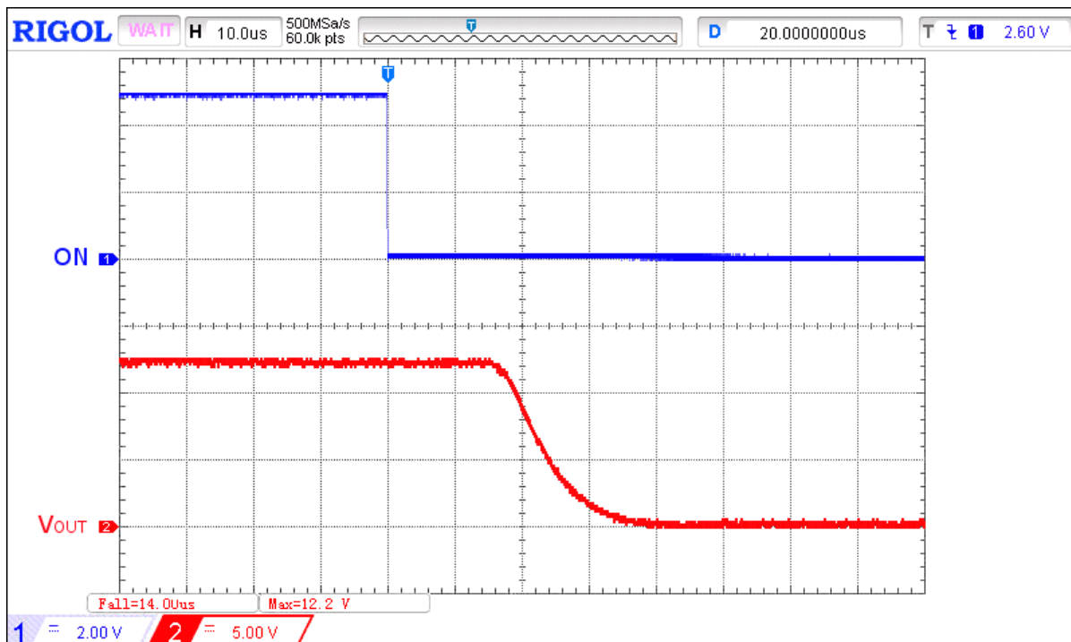
Figure 6. Typical Turn OFF operation waveform for V_{IN} = 12 V, C_{SLEW} = 10 nF, no C_{LOAD} , R_{LOAD} = 100 Ω
