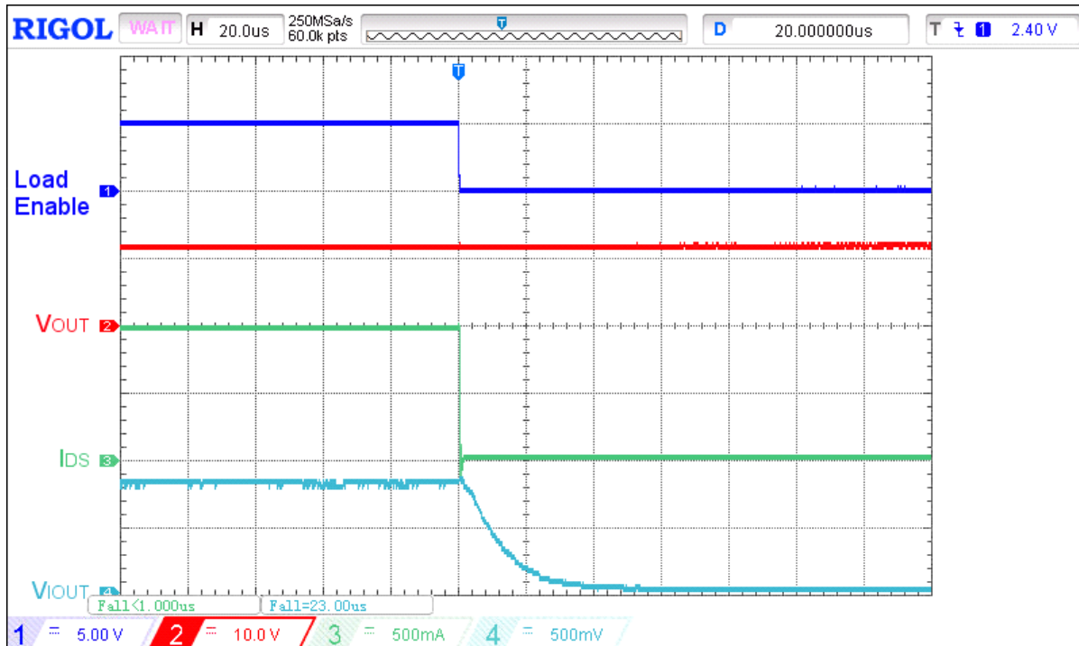
Figure 18. Typical I OUT response time waveform for V IN = 12 V, C LOAD = 10 μF, R LOAD = 12 Ω C IOUT = 0.18 nF, R IOUT = 84.5 kΩ, Load step 1 A to 0 A
