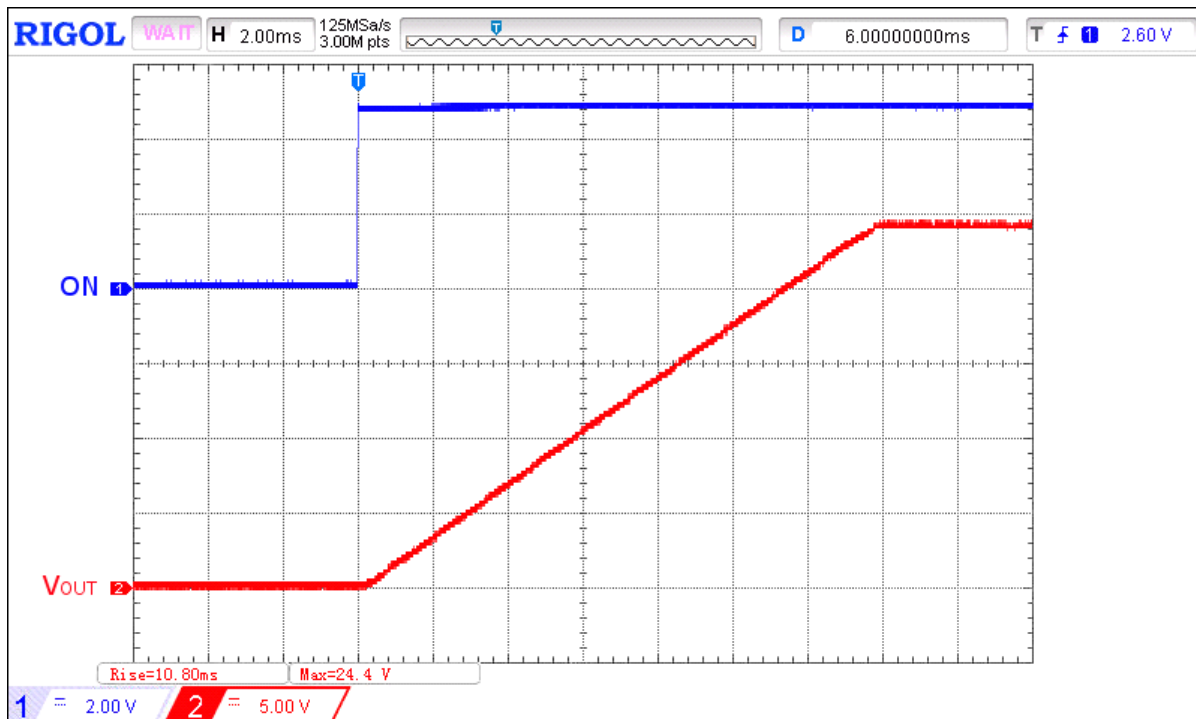
Figure 5. Typical Turn ON operation waveform for V_{IN} = 24 V, C_{SLEW} = 18 nF, C_{LOAD} = 10 μF, R_{LOAD} = 100 Ω
