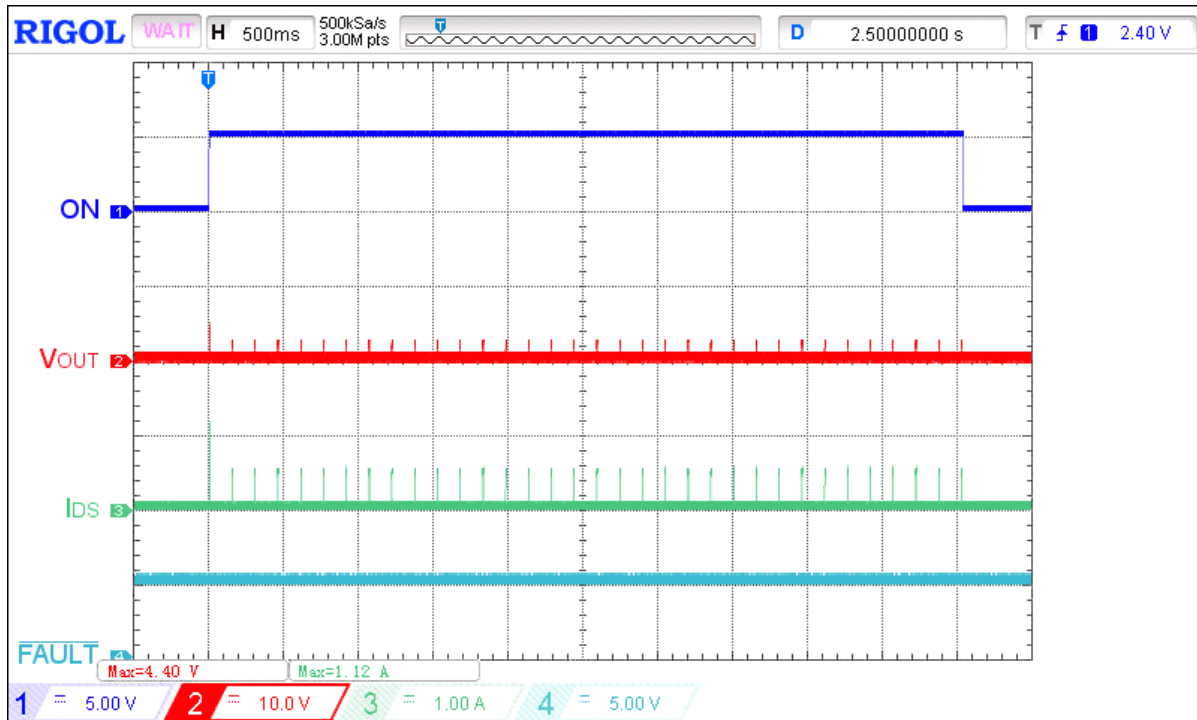
Figure 21. Typical SOA waveform during power up on heavy load for V IN = 12 V, C LOAD = 10 μF, R SET = 30.1 kΩ, R LOAD = 3.5 Ω
