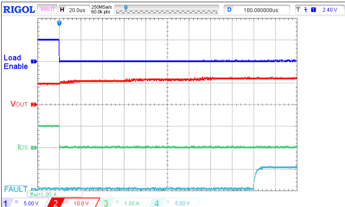
Figure 14. Typical FAULT de-assertion waveform for V IN = 12 V, C LOAD = 10 μF, I ACL = 1 A, R SET = 91 kΩ, switch out 9 Ω load
