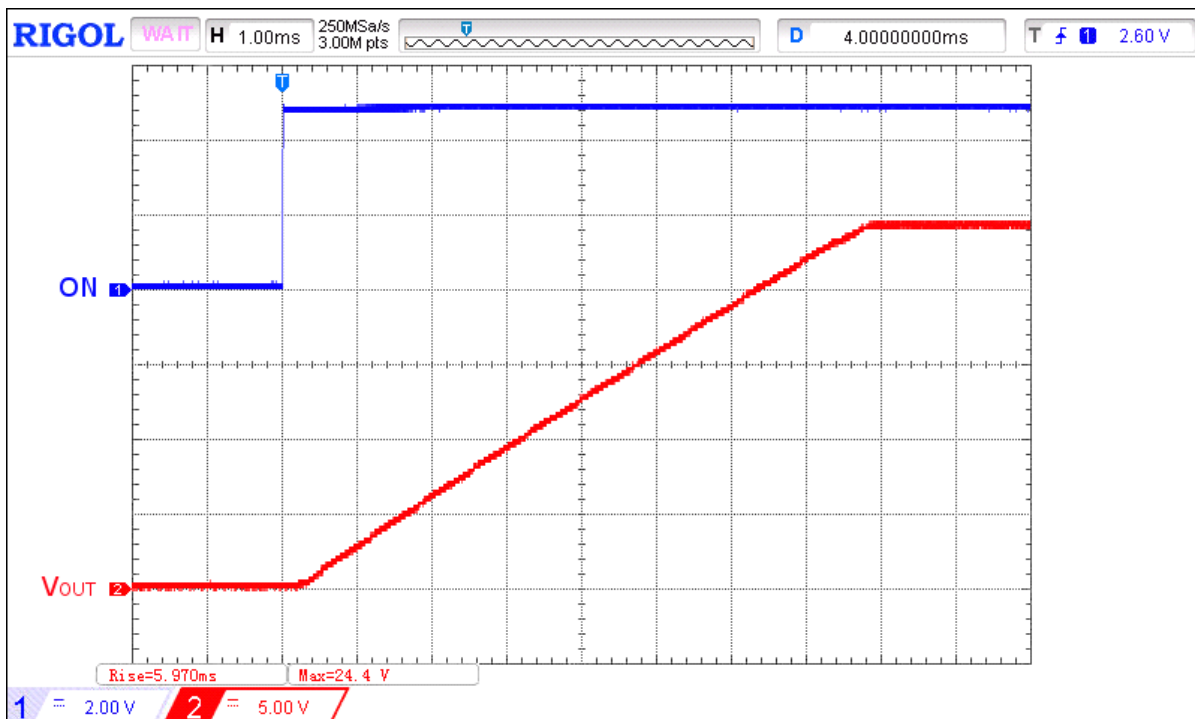
Figure 4. Typical Turn ON operation waveform for V_{IN} = 24 V, C_{SLEW} = 10 nF, C_{LOAD} = 10 μF, R_{LOAD} = 100 Ω
