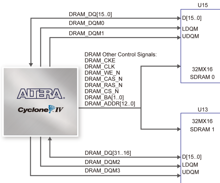
Figure 4-34 Connections between FPGA and SDRAM
