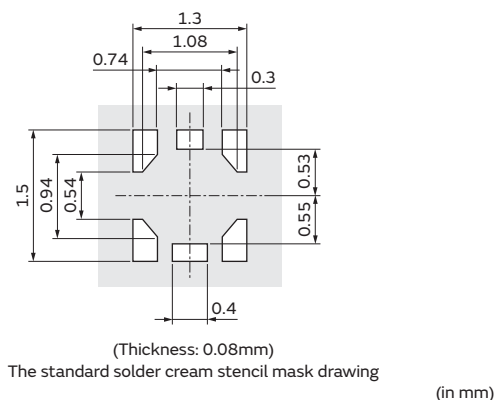
Standard Stencil Mask Pattern
