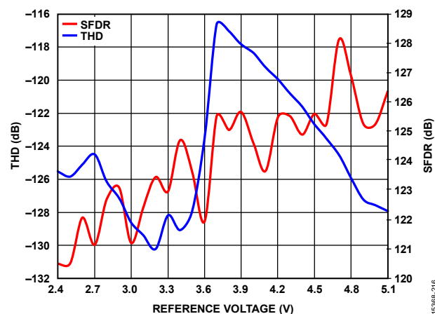
Figure 21. THD and SFDR vs. Reference Voltage, f_{IN} = 1 kHz
