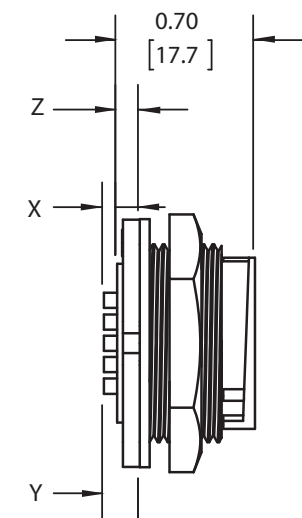
14X80-XXG-3XX PANEL MOUNT CONNECTOR CRIMP
