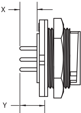
14XXX-XXG-3XX PANEL MOUNT CONNECTOR PC TAIL
