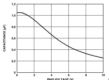
Figure 26. Capacitance vs. Bias Voltage Characteristics
