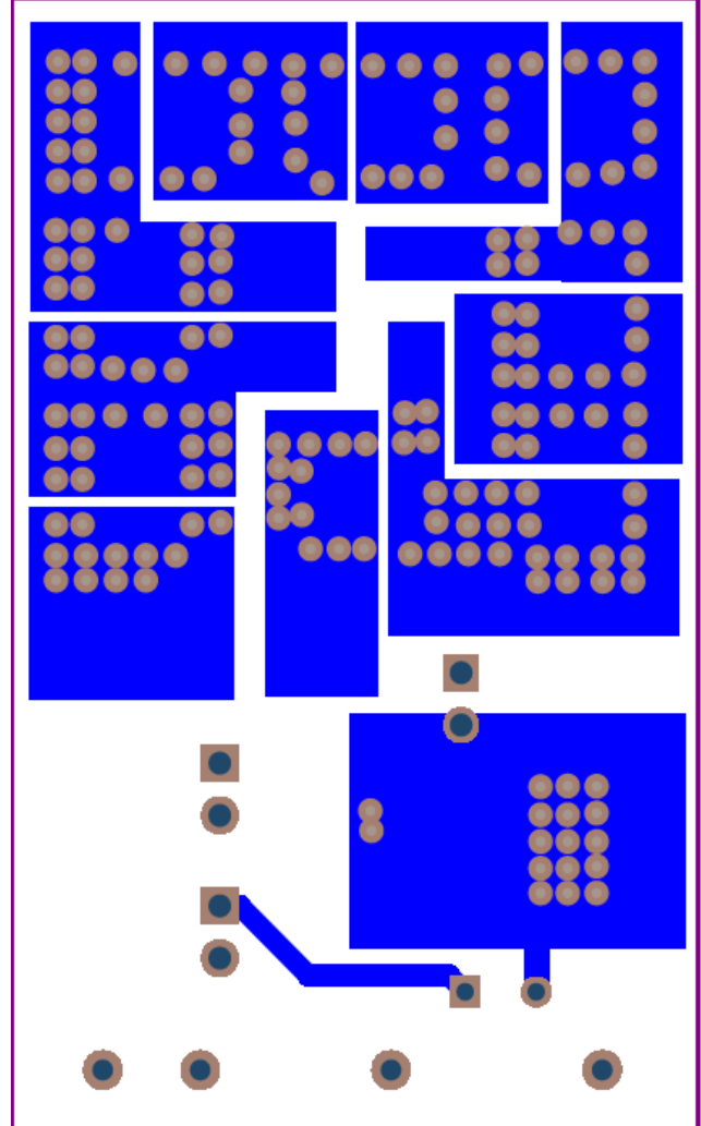
Figure 5 Layout bottom
