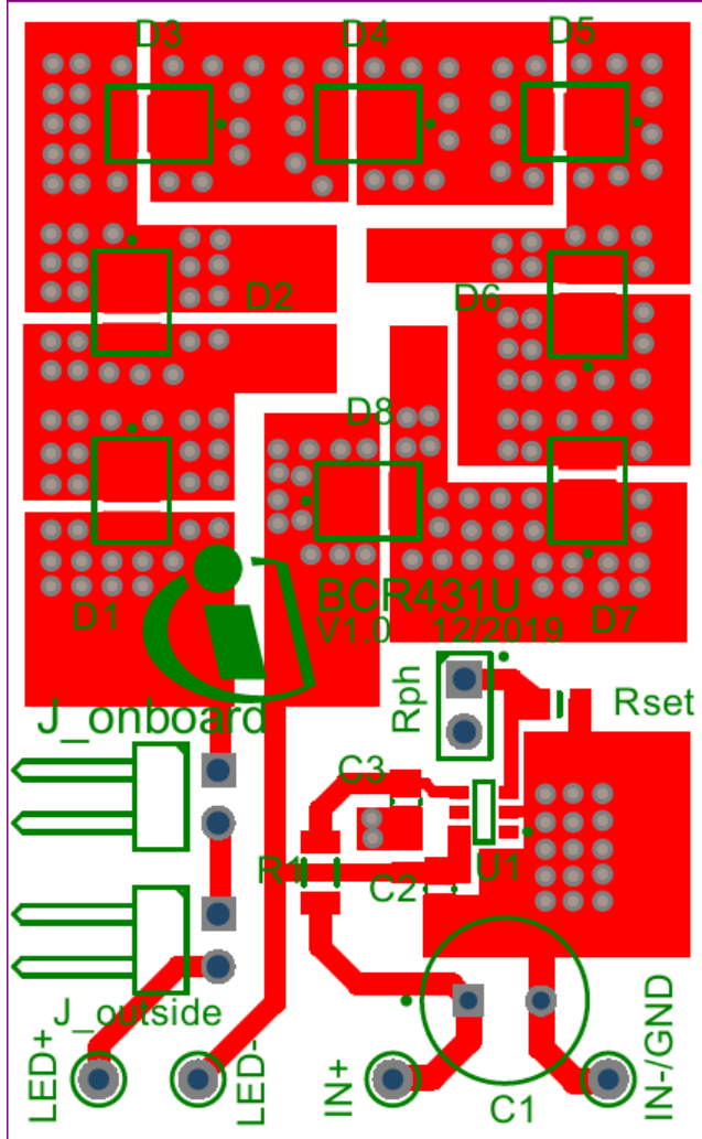
Figure 4 Layout top
