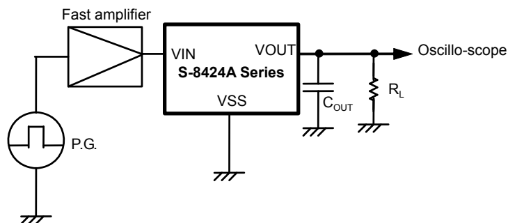
Figure 15 Test Circuit
