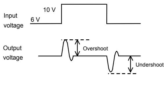
Figure 14 Power Supply Variation: 6 V and 10 V Square Waves
