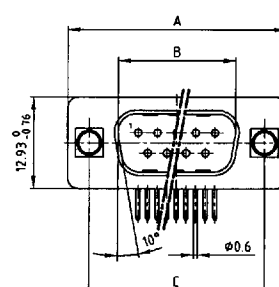
Plug connector
