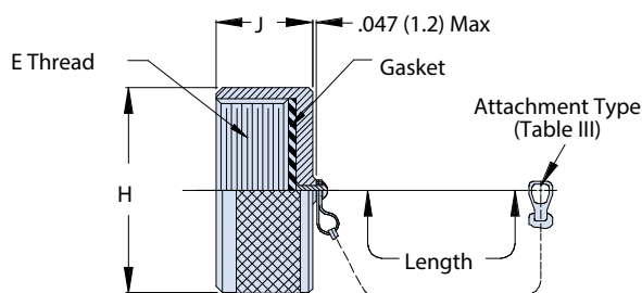
660-005 Receptacle Cover
