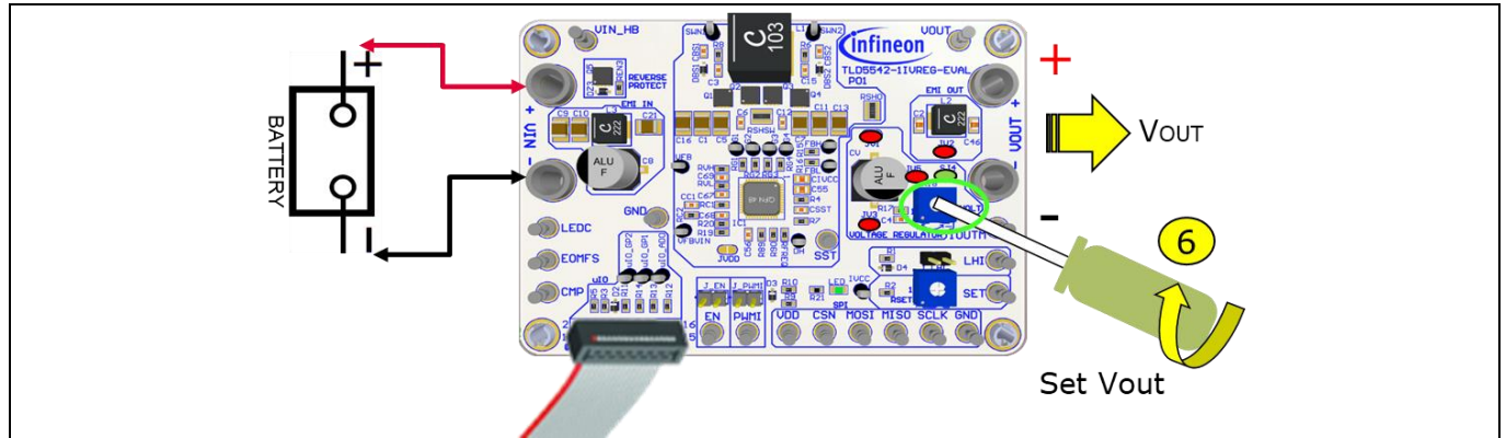
Figure 11 Voltage regulator with µIO stick: Adjust full scale (100% ADIM) V_{OUT}
