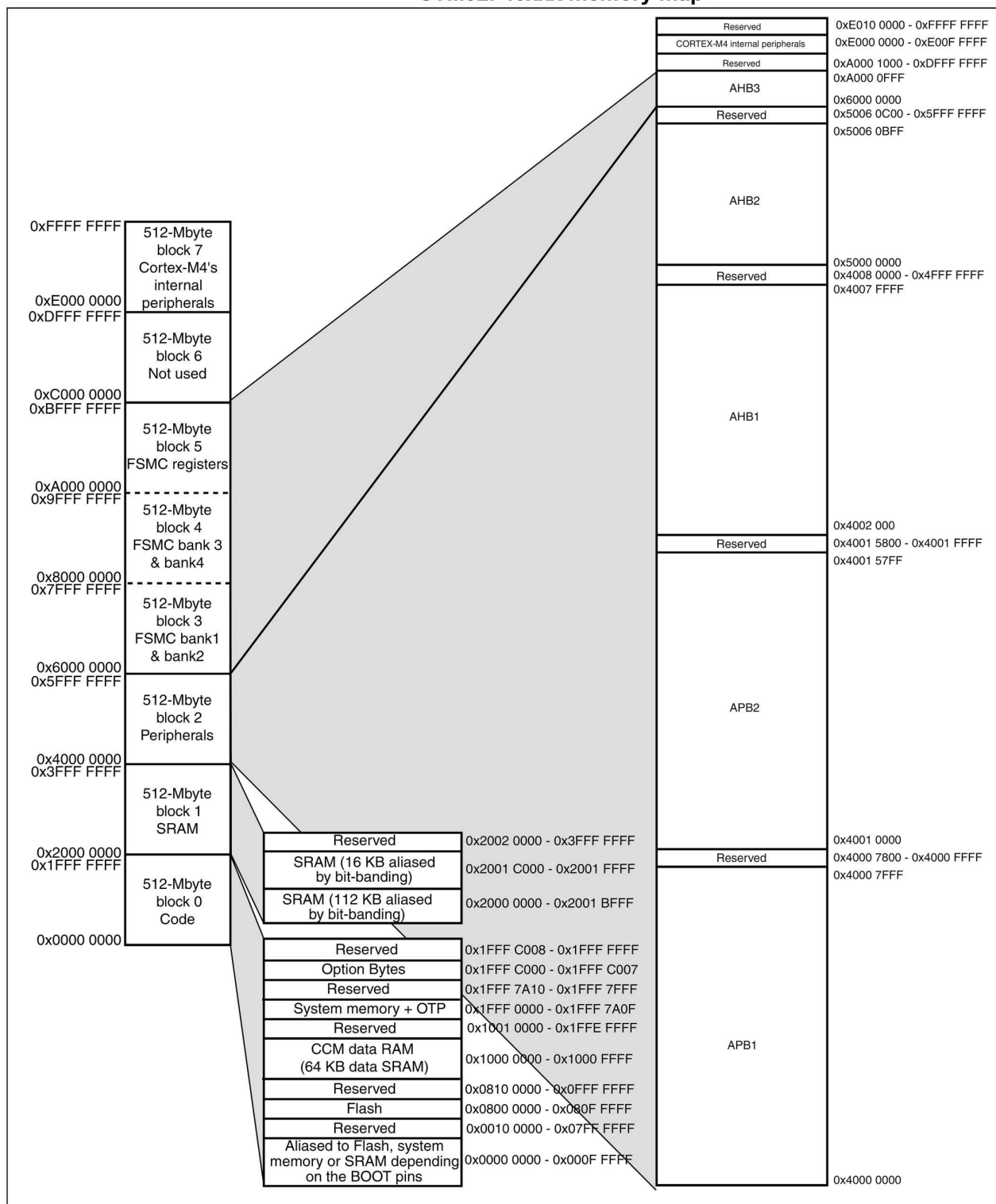
STM32F40xxx memory map
