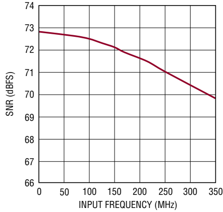
LTM9006-14: SNR vs Input Frequency, -1dBFS, 2V Range, 25Mps
