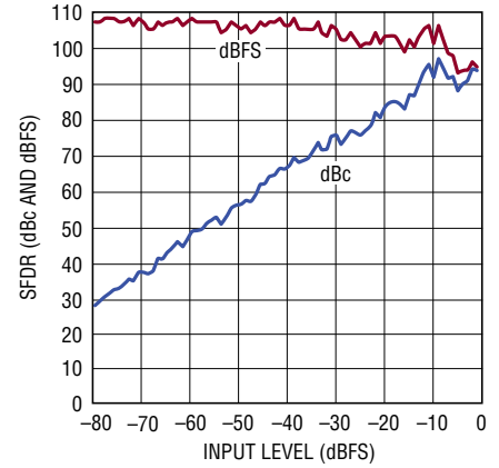
LTM9006-14: SFDR vs Input Level, f_{IN} = 70\text{MHz} , 2V Range, 25Mps
