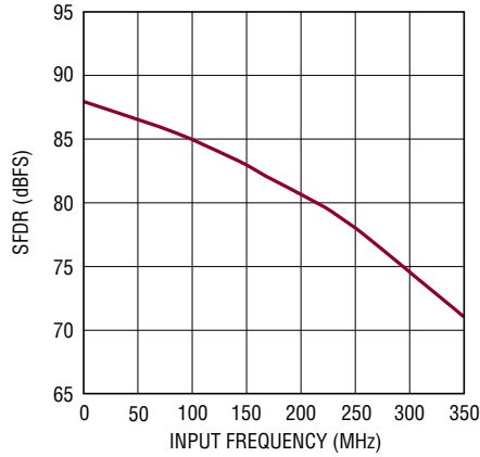
LTM9006-14: SFDR vs Input Frequency, -1dBFS, 2V Range, 25Mps
