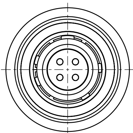
S10YCR-P04XFG0-0000 Mechanical coding: C Color coding: blue
