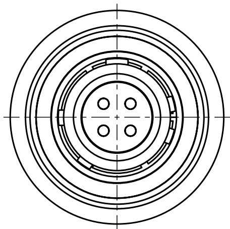
S10YBR-P04XFG0-0000 Mechanical coding: B Color coding: red
