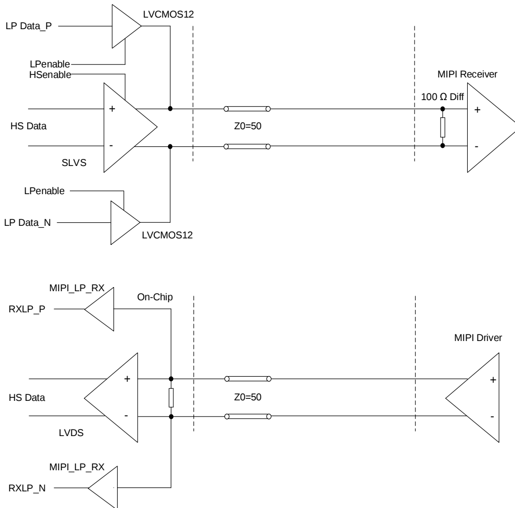
Figure 3.6. MIPI Interface
