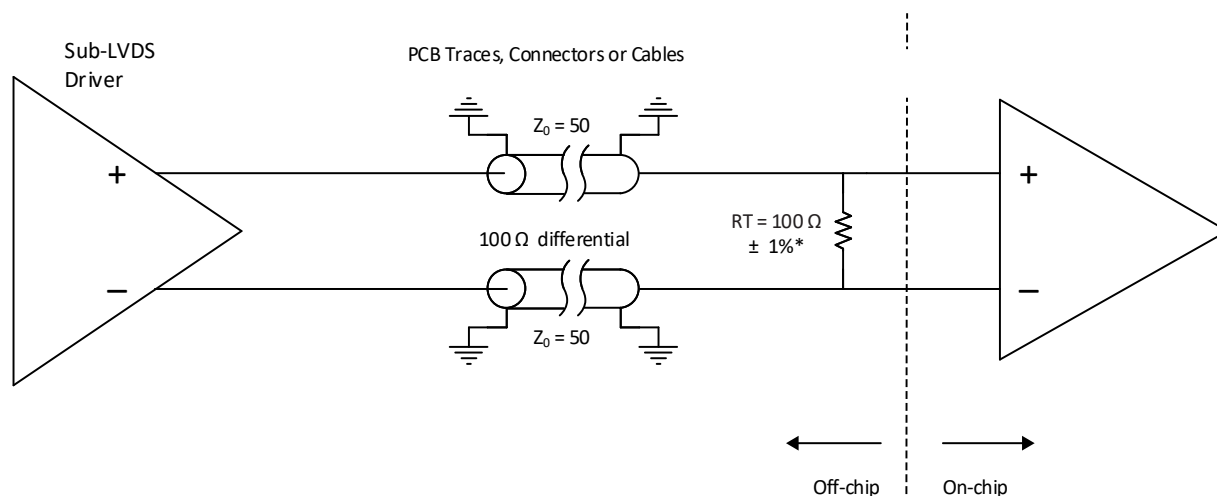
Figure 4.3. SubLVDS Input Interface
