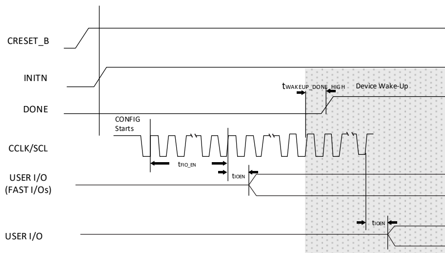
Figure 4.21. Slave SPI/I²C/I³C Wake-Up Timing
