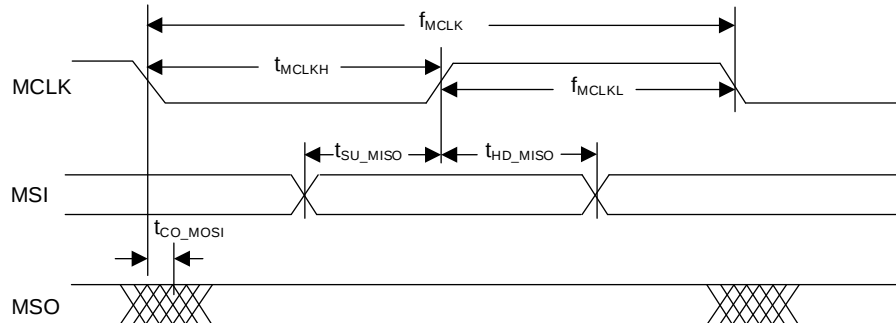
Figure 3.18. Master SPI Configuration Timing
