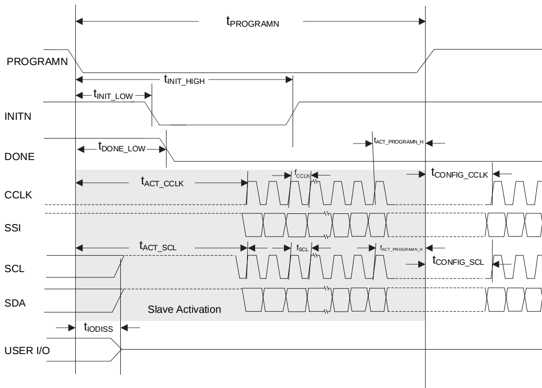
Figure 4.16. Slave SPI/I²C/I³C PROGRAMN Timing
