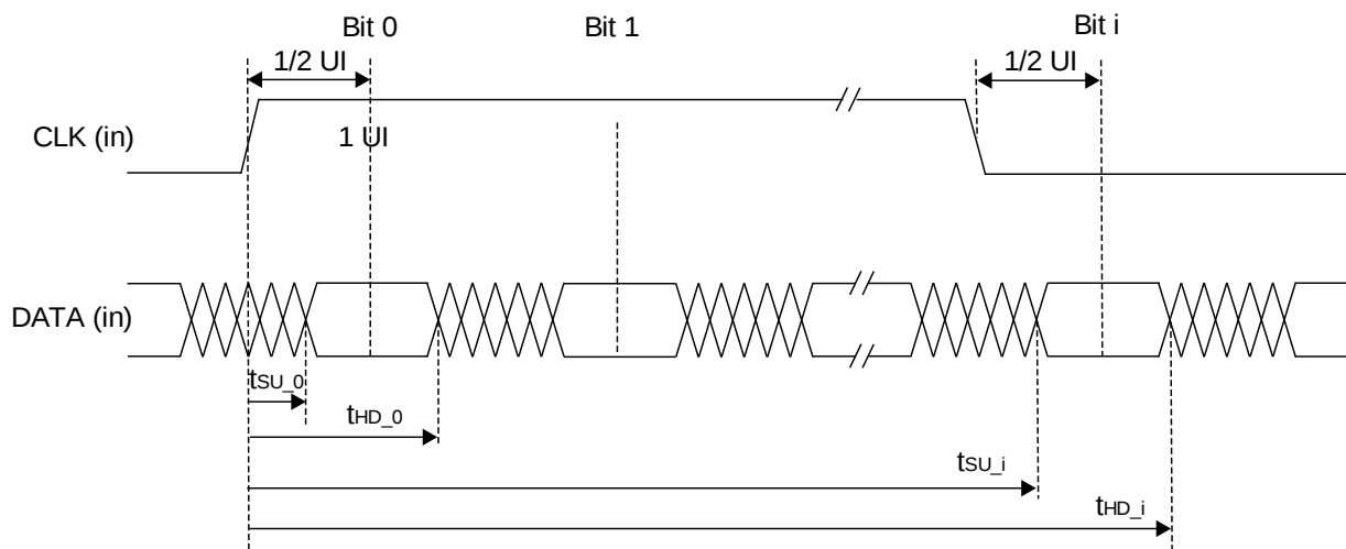
Figure 4.11. Receiver DDRX71_RX Waveforms
