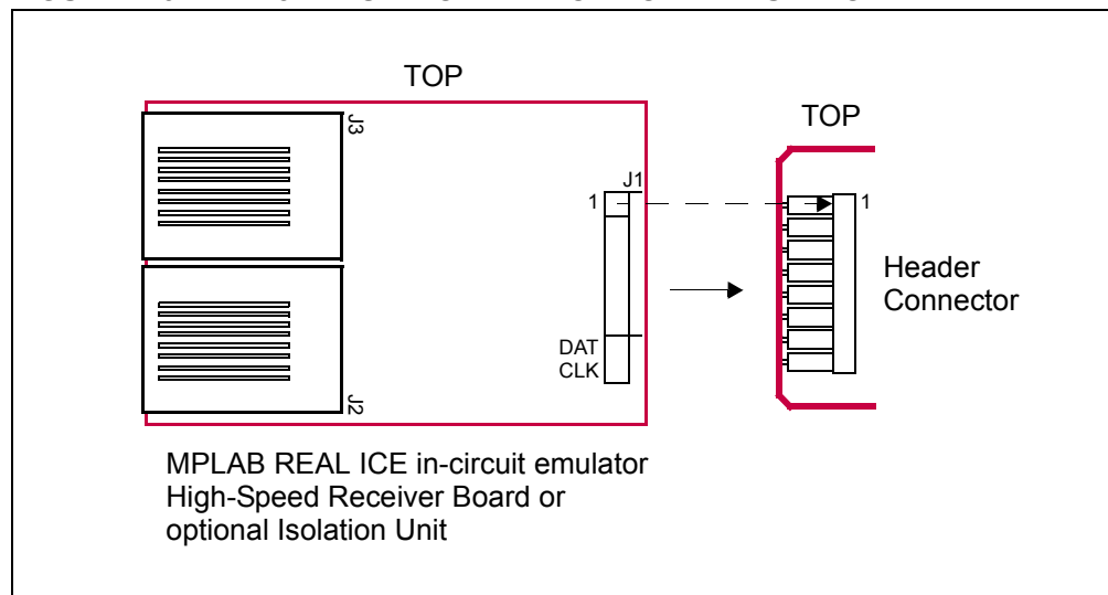
FIGURE B-3: 8-PIN SIL CONNECTION TO AN EMULATOR
