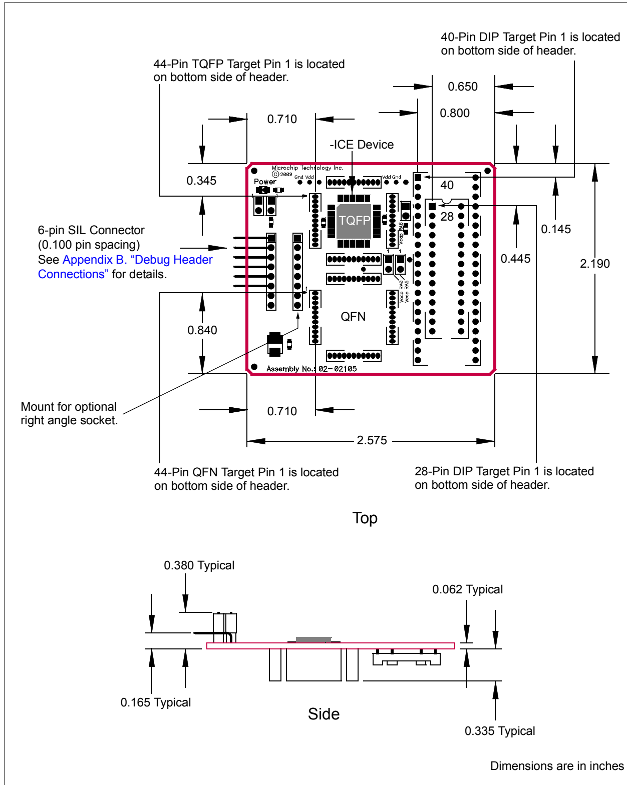
FIGURE 3-16: DIMENSIONS - AC244048
