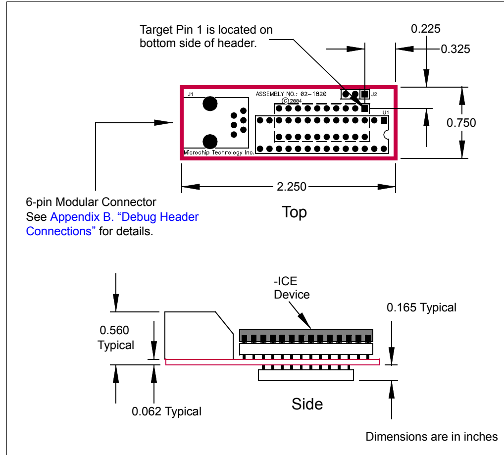
FIGURE 2-5: DIMENSIONS – AC162060
