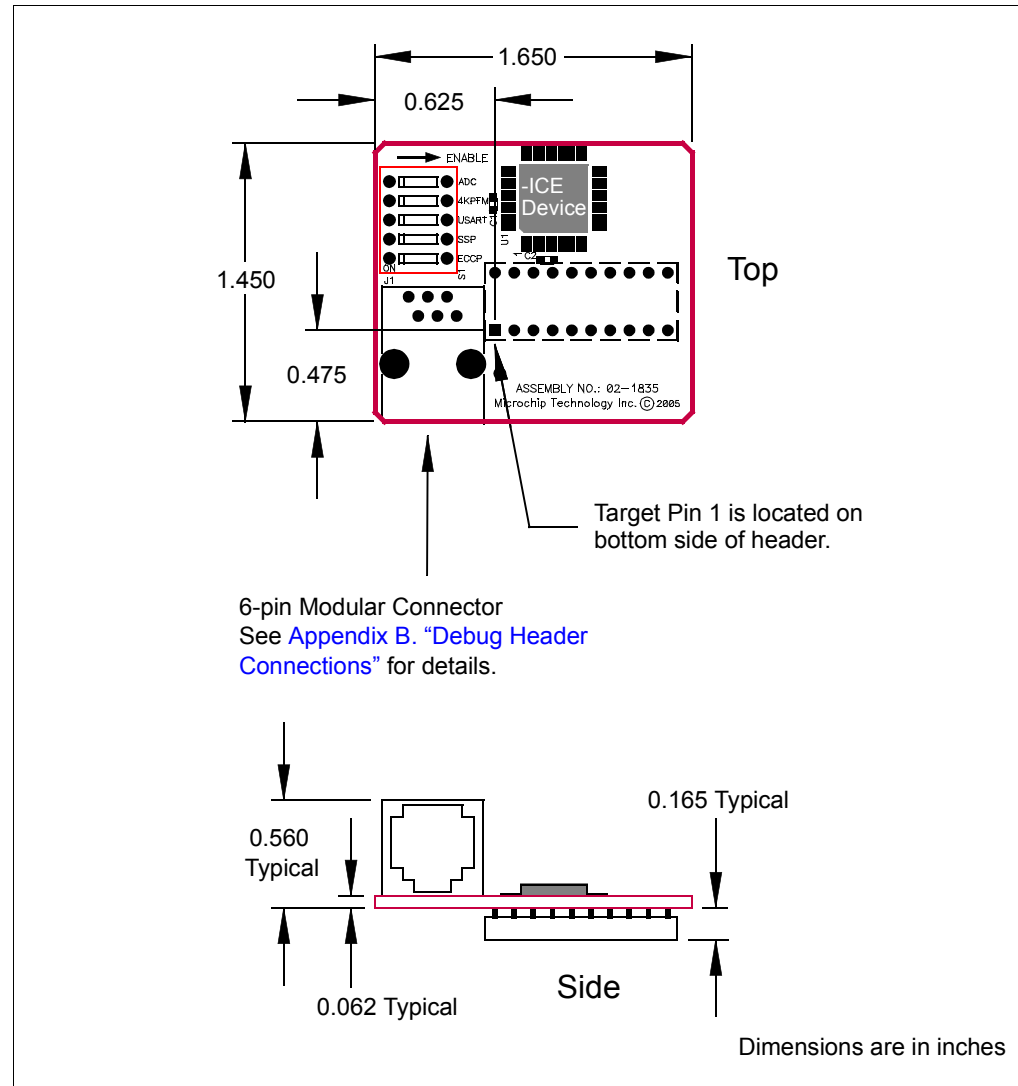
FIGURE 2-7: DIMENSIONS – AC162061
