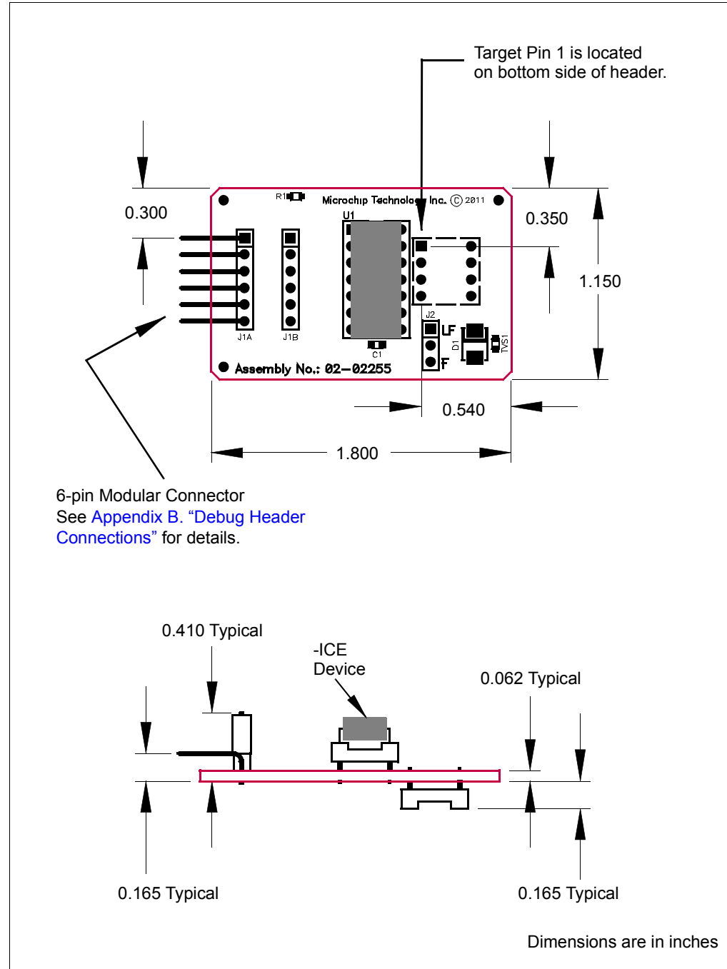
FIGURE 2-12: DIMENSIONS - AC244045
