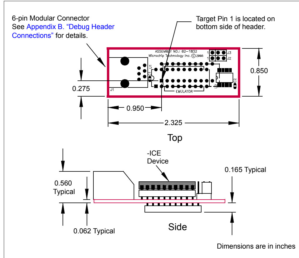
FIGURE 2-8: DIMENSIONS – AC162066
