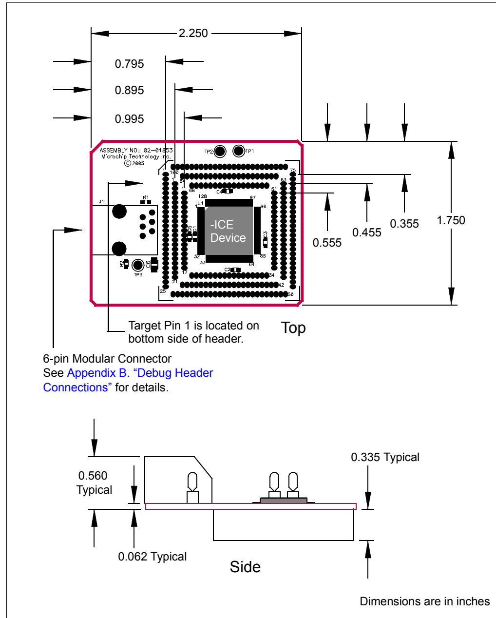
FIGURE 3-3: DIMENSIONS – AC162064
