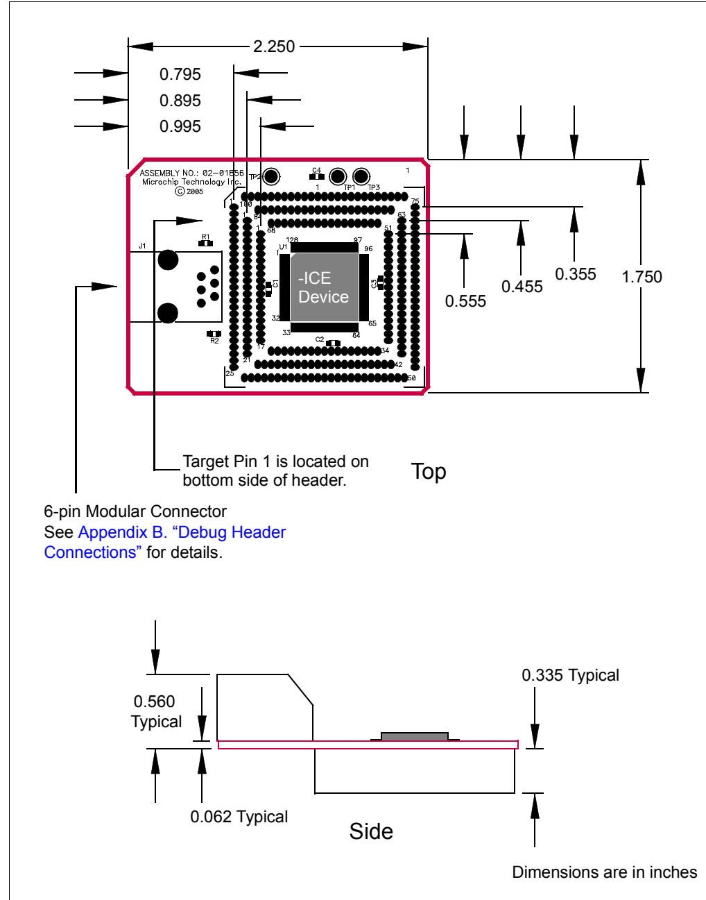
FIGURE 3-4: DIMENSIONS – AC162065
