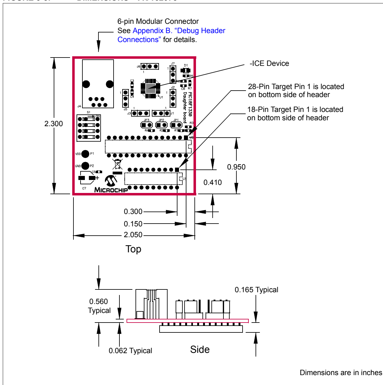
FIGURE 3-8: DIMENSIONS – AC162078
