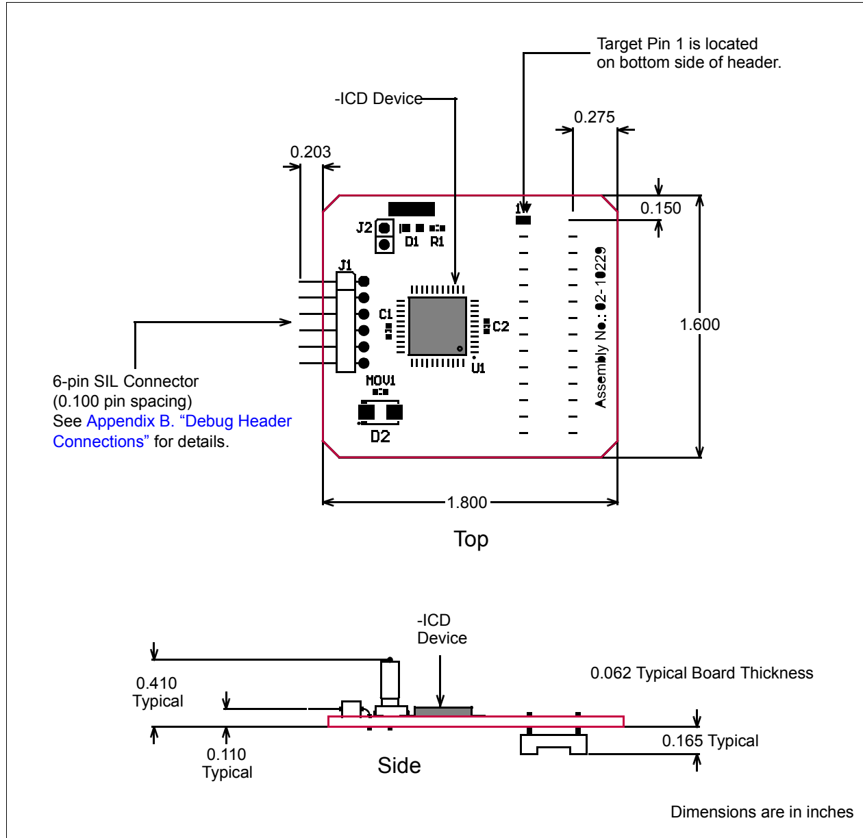
FIGURE 2-14: DIMENSIONS - AC244062
