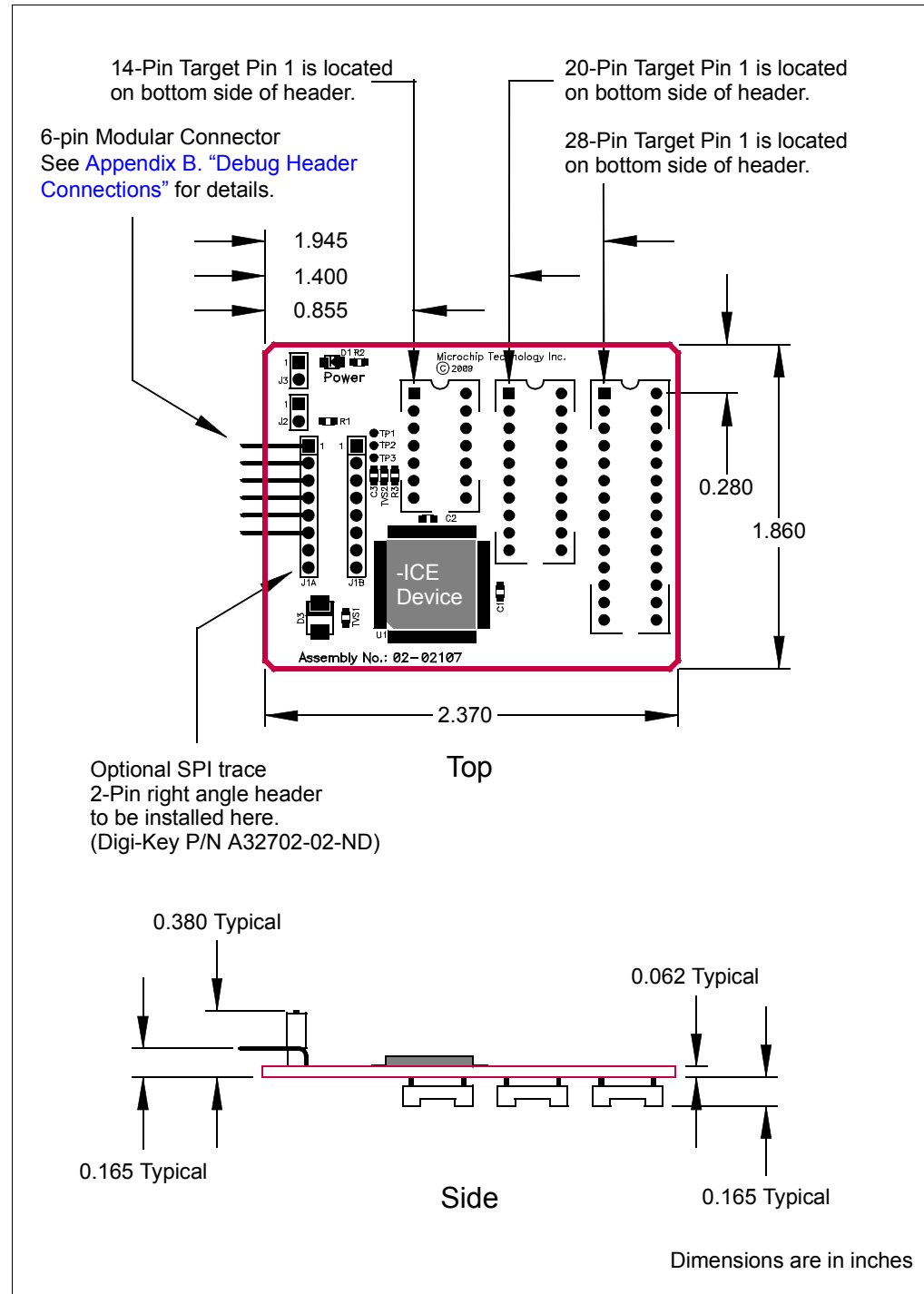
FIGURE 2-11: DIMENSIONS - AC244028
