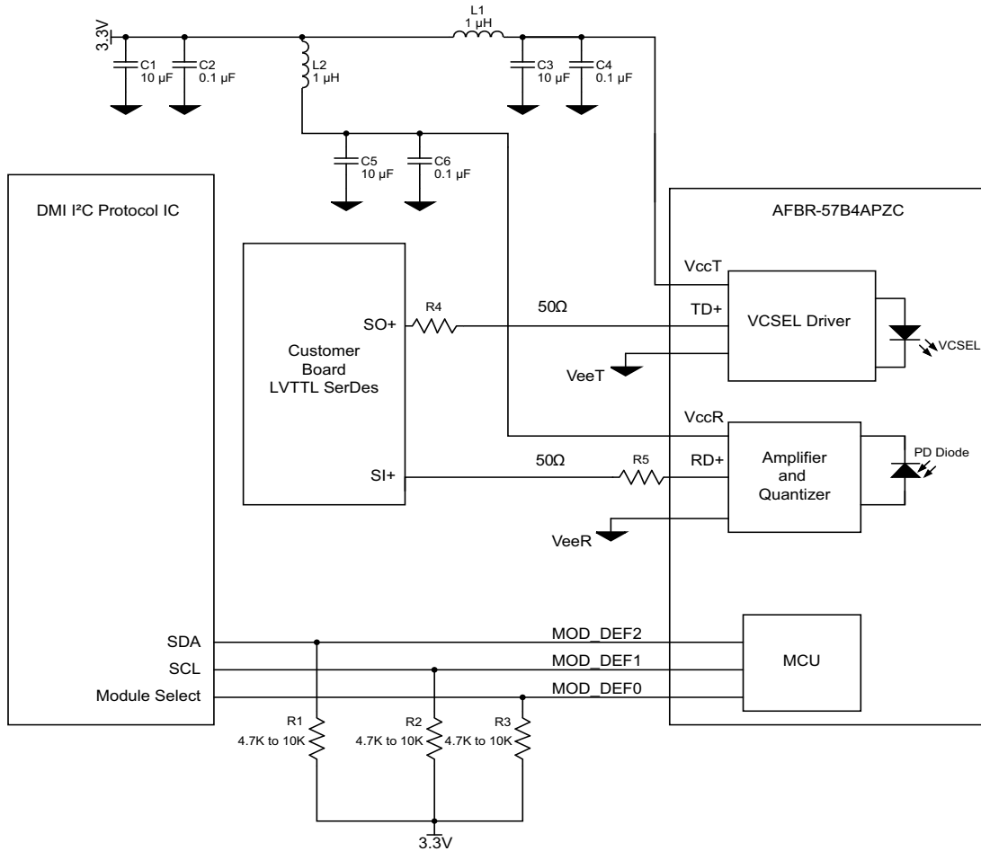
Figure 3: Recommended Application Circuitry
