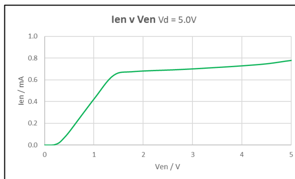
Figure 12: I_{en} v V_{en} V_d = 5.0V
