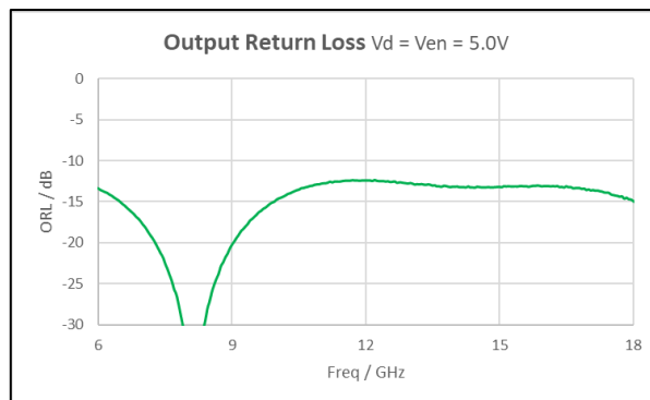
Figure 8: Output Return Loss V_d = V_{en} = 5.0V
