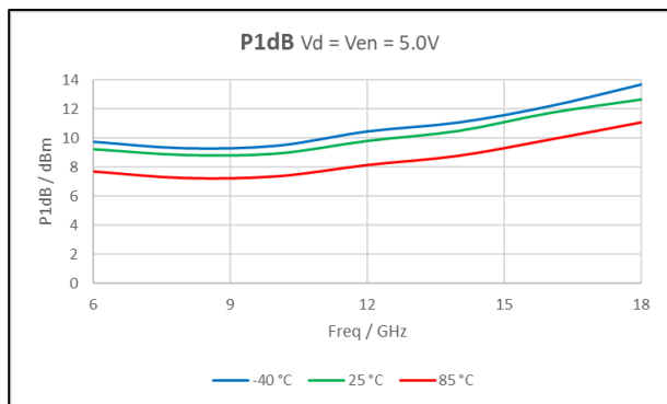
Figure 35: P1dB V_d = V_{en} = 5.0V
