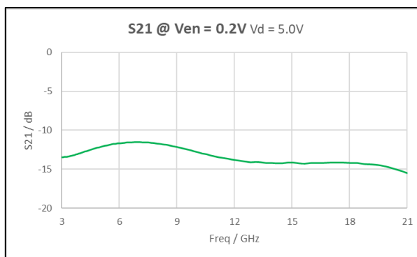
Figure 10: S_{21} @ V_{en} = 0.2V V_d = 5.0V
