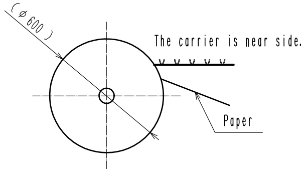
Fig.1 Reel drawing
