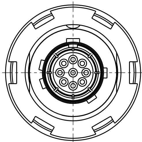
G80YBR-P09UC00-000L Mechanical coding: B Color Coding: red
