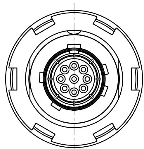
G80YCR-P09UC00-000L Mechanical coding: C Color Coding: blue
