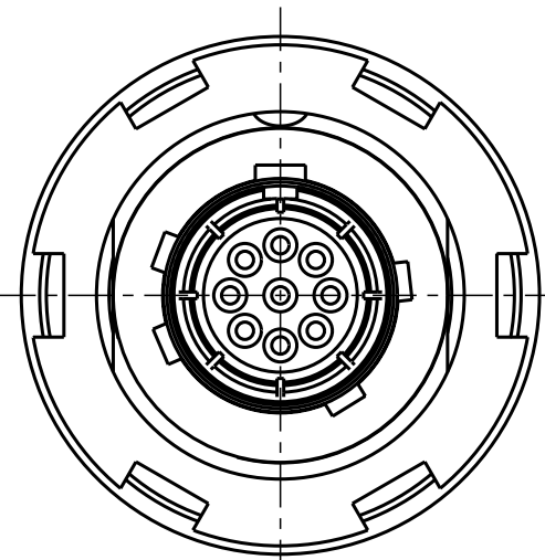
G80YDR-P09UC00-000L Mechanical coding: D Color Coding: green
