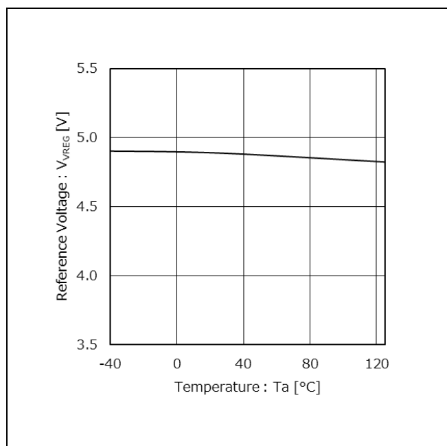
Figure 9. Reference Voltage vs Temperature (VCC = 12 V, V_{EN} = 3.3\text{ V} , V_{PWM} = 0\text{ V} )
