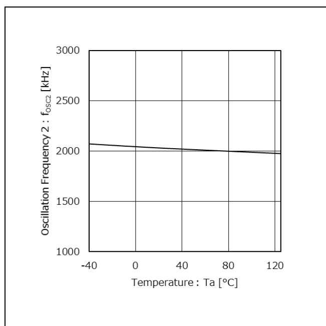
Figure 11. Oscillation Frequency 2 vs Temperature (@2000 kHz, VCC = 12 V, V_{EN} = 3.3\text{ V} , R_{RT} = 3.6\text{ k}\Omega )
