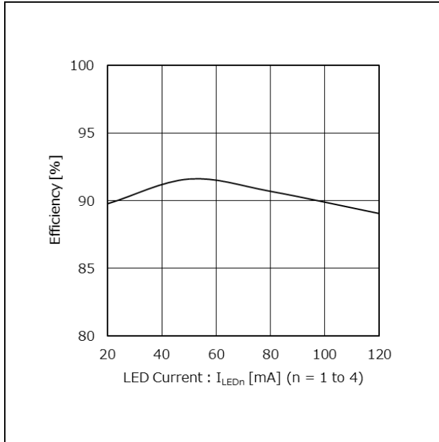
Figure 14. Efficiency vs LED Current( n = 1 to 4 ) (Buck-Boost Application) ( T_a = 25\text{ }^{\circ}\text{C} , V_{CC} = 12\text{ V} , V_{EN} = 3.3\text{ V} , V_{PWM} = V_{VREG} , 4 LED loads per channel, all channels have loads)
