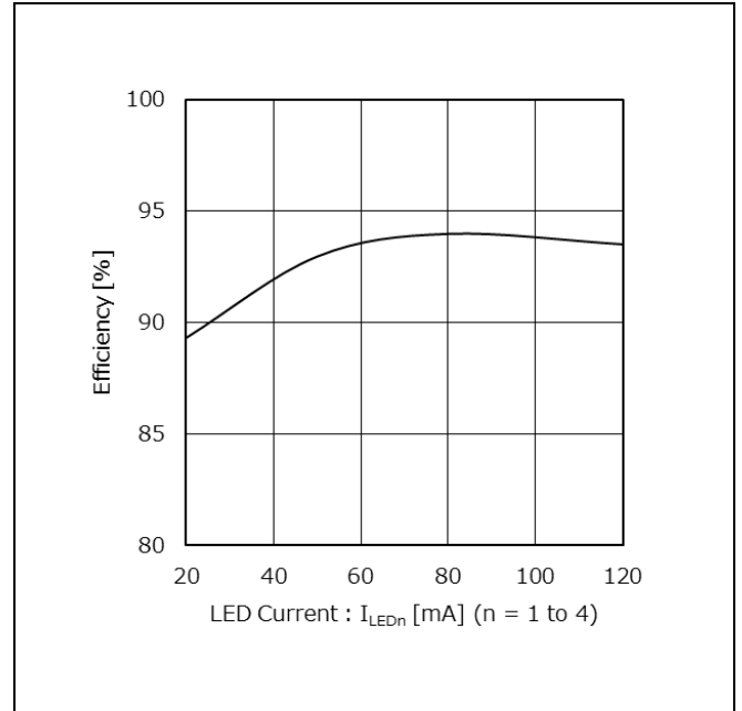
Figure 15. Efficiency vs LED Current( n = 1 to 4 ) (Boost Application) ( T_a = 25\text{ }^{\circ}\text{C} , V_{CC} = 12\text{ V} , V_{EN} = 3.3\text{ V} , V_{PWM} = V_{VREG} , 8 LED loads per channel, all channels have loads)
