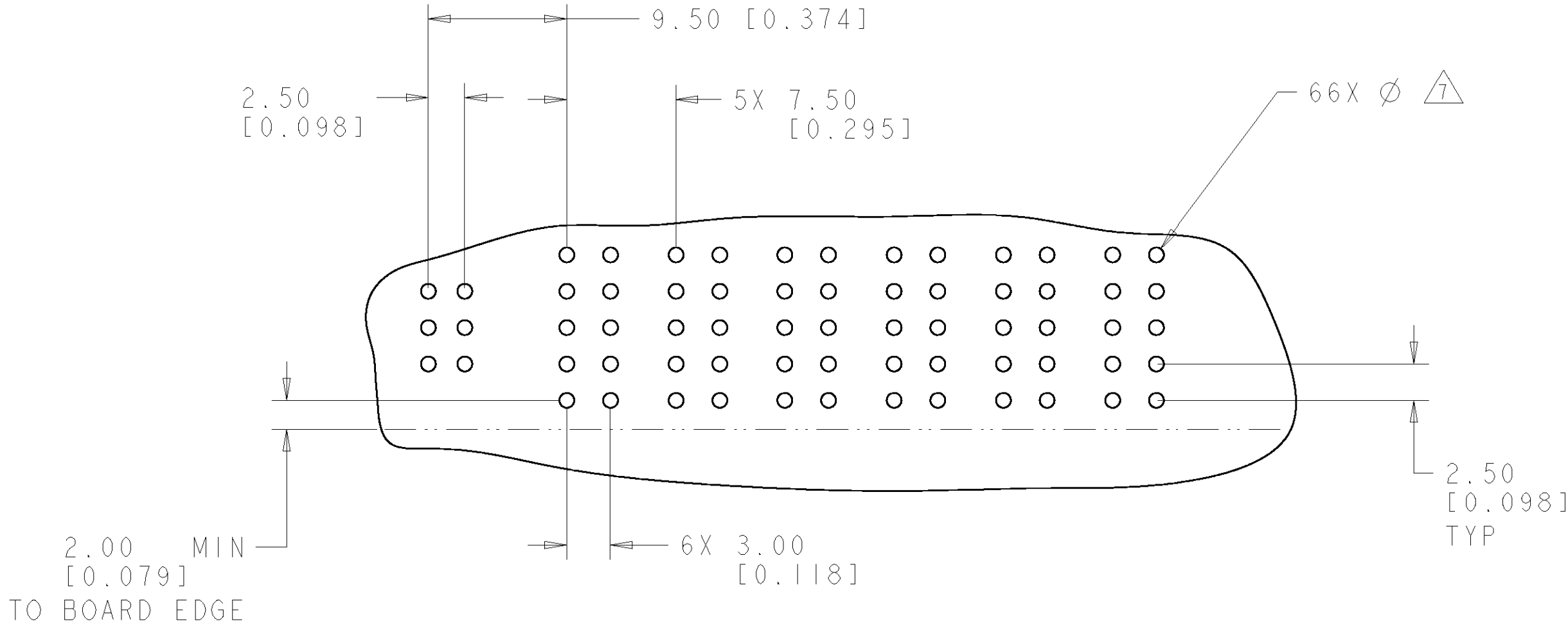
PRINTED CIRCUIT LAYOUT SCALE 3:1
