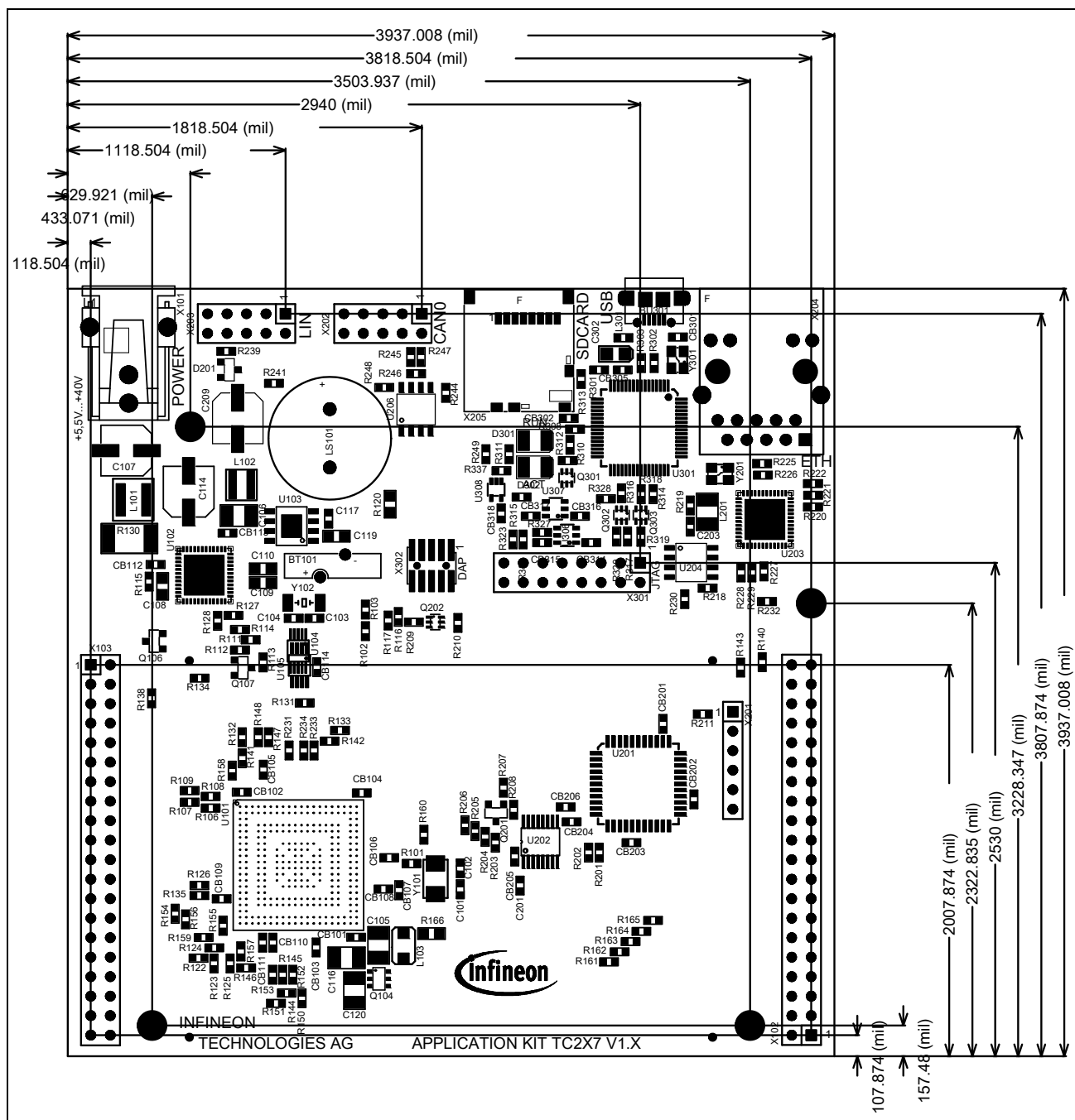
Figure 6-8 Dimensioning (mil)
