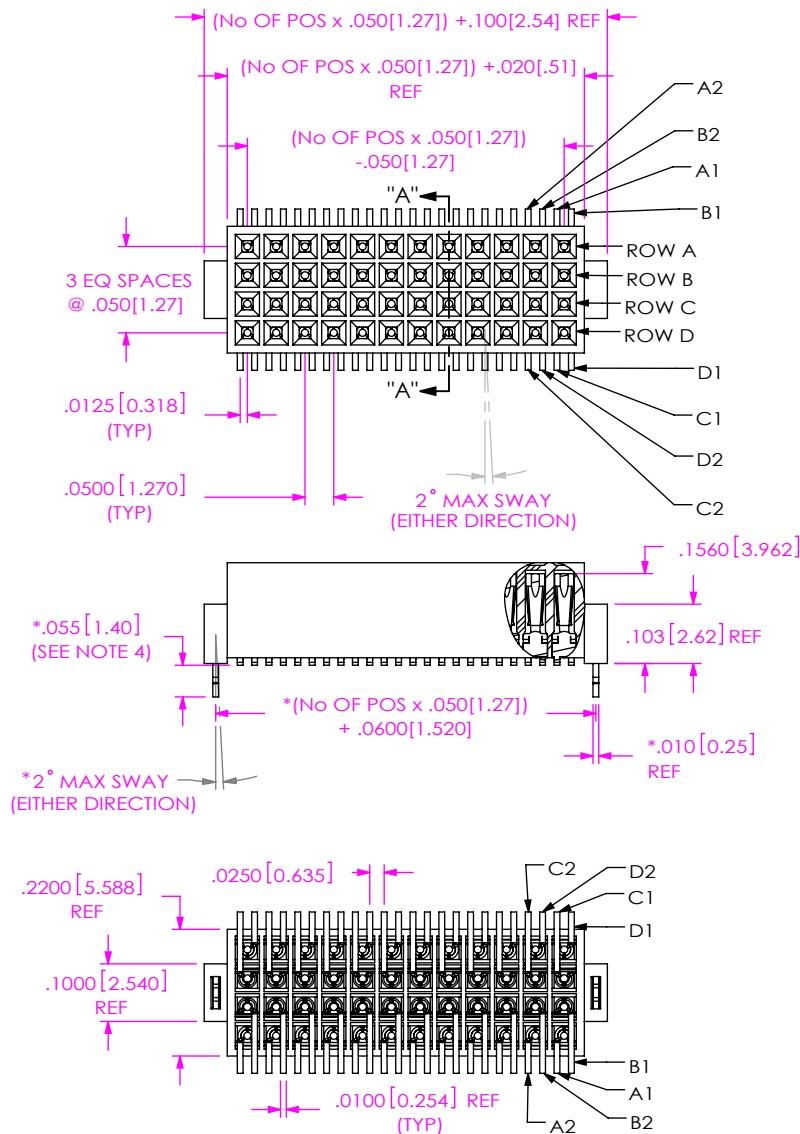
FIG 1 FOLC-1XX-XX-X-Q-LC SHOWN * = -LC DIMENSIONS
