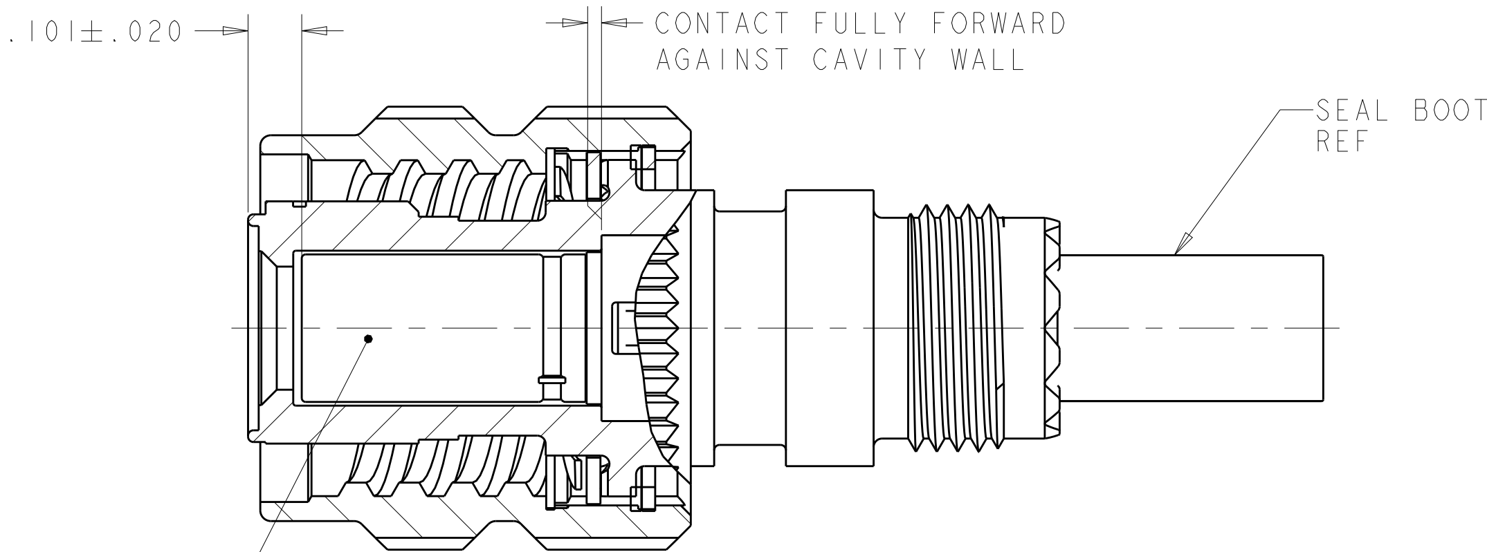
SECTION X-X
