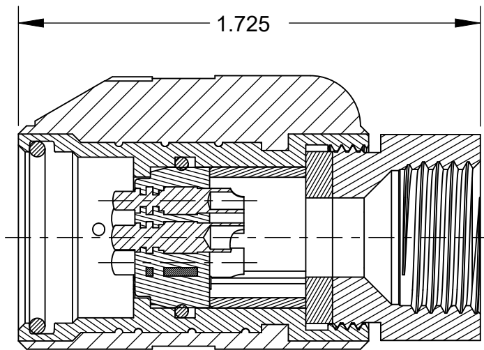
SECTION Z-Z
