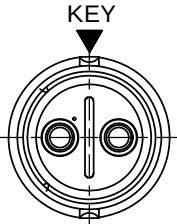
WIRING END W6380-2PG-P-3XX SHOWN WITHOUT HARDWARE
