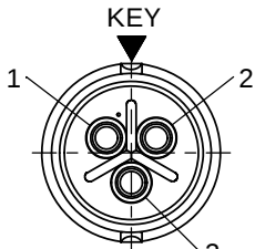
WIRING END W6380-3PG-P-3XX
