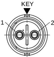
WIRING END W6380-2PG-P-3XX
