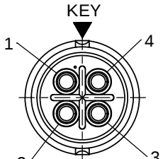
WIRING END W6380-4PG-P-3XX
