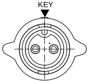
MATING FACE W6380-2PG-P-3XX SHOWN
