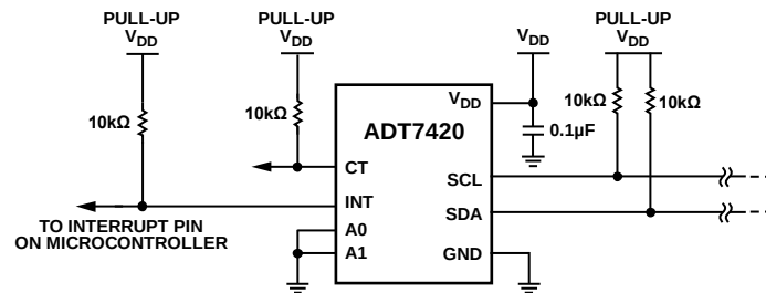
Figure 13. Typical I²C Interface Connection
