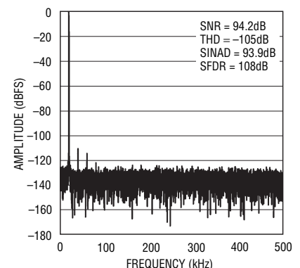
16k Point FFT f_s = 1\text{MSPS} , f_{\text{IN}} = 20\text{kHz}
