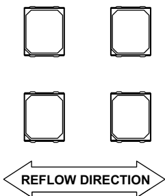
Figure 24: Recommended Board Reflow Direction
